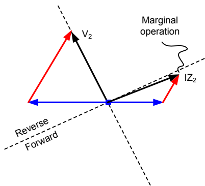
Fig. 29. Superimposed negative-sequence voltages and currents for the simultaneous forward AG and reverse BG faults.
