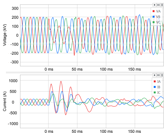
Fig. 31. Phase voltages and currents recorded by the relay at the wind farm.
