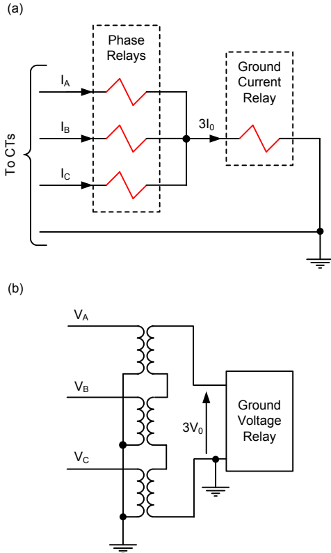
Fig. 7. Obtaining 3I_0 and 3V_0 relay input quantities with connections of secondary wires. Zero-sequence current relay in the return CT lead (a); zero-sequence voltage relay connected to open-delta VTs (b).
