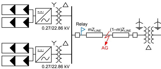
Fig. 35. One-line diagram of a power system with IBRs.
