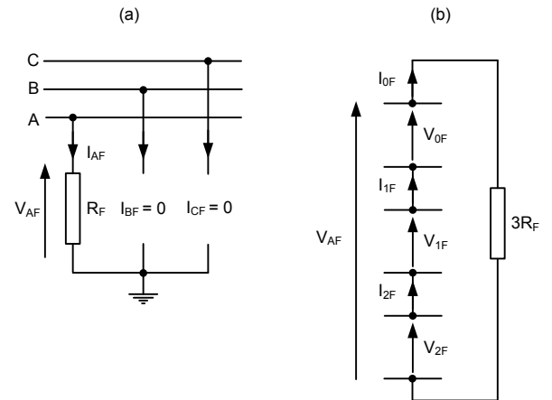
Fig. 5. AG fault as an example of an unbalance: physical network (a); resulting connection of sequence networks (b).
