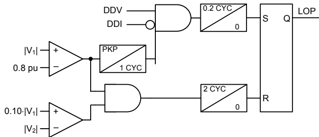
Fig. 19. Simplified LOP logic.
