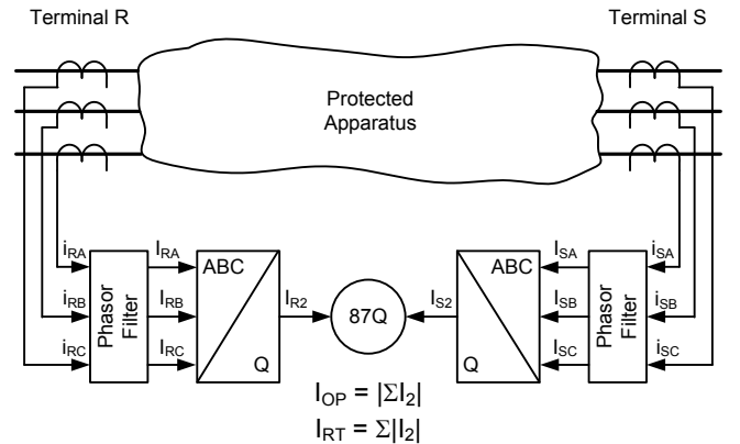
Fig. 13. Negative-sequence differential scheme.
