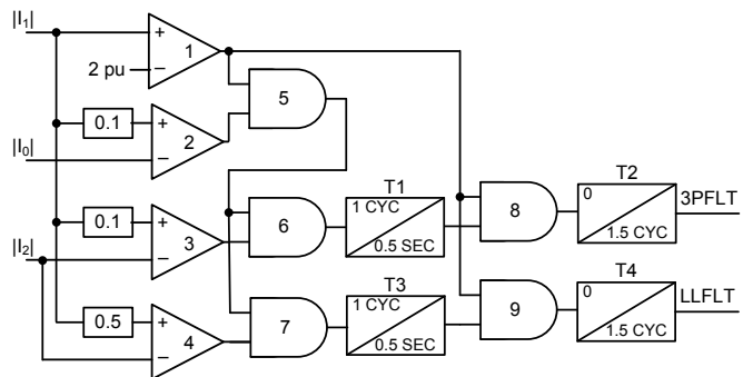
Fig. 23. Logic securing sequence elements for spurious sequence currents caused by CT saturation.
