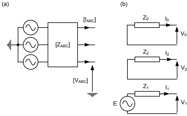
Fig. 3. Sequence networks for a traditional three-phase source.
