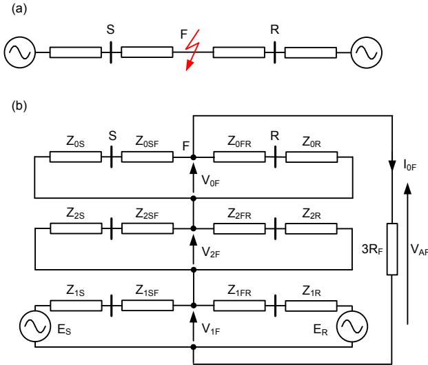
Fig. 6. Simple power system (a) represented with sequence networks for an AG fault (b).
