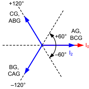
Fig. 11. The principle of fault type identification using negative- and zero-sequence currents (ABC phase sequence).
