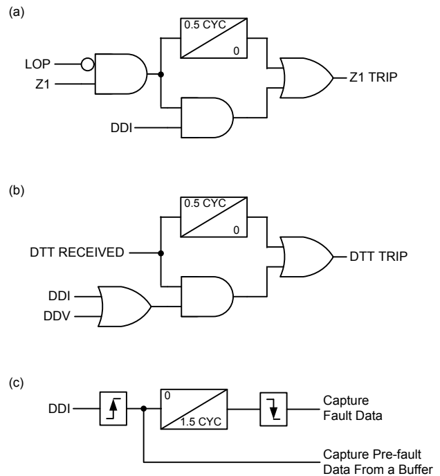
Fig. 17. Sample applications of disturbance detection logic: distance Z1 trip logic (a); DTT supervision for improved security against channel noise (b); event reporting pre-fault and fault data capture (c).
