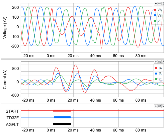
Fig. 34. Response of the relay based on incremental quantities [16] to the fault in Fig. 31 with correct directional (TD32F) and phase-selection (AGFLT) decisions.
