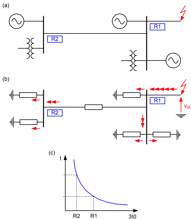
Fig. 16. The zero-sequence current is higher when measured at the fault (Relay R1) and lower when measured further away from the fault (Relay R2); one-line diagram (a); zero-sequence network and current flow (b); inverse-time overcurrent characteristic (c).
