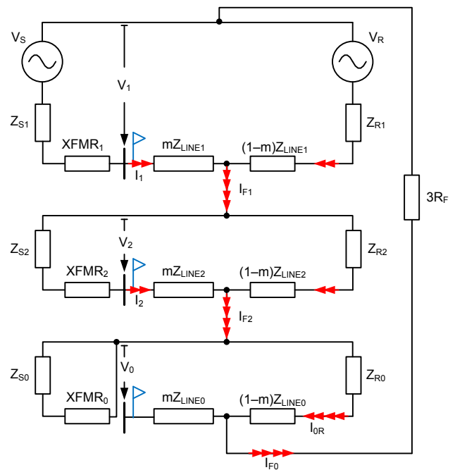
Fig. 37. Sequence network diagram for an AG fault for the system shown in Fig. 35 but with the IBR source replaced by a conventional power source.
