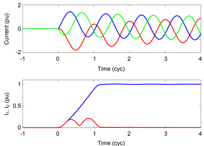
Fig. 22. Example of the spurious transient negative-sequence current (red trace) for a three-phase balanced fault.
