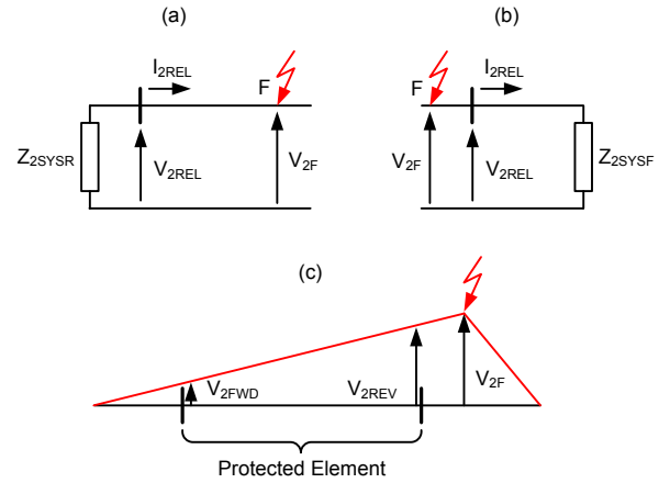
Fig. 8. Principle of the negative-sequence directional element: forward fault (a); reverse fault (b); voltage profile for an external fault (c).
