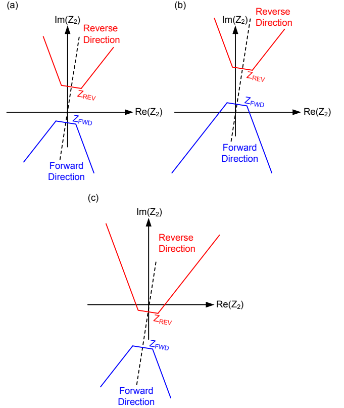
Fig. 10. Negative-sequence directional element without bias (a) and with forward (b) and reverse (c) bias.
