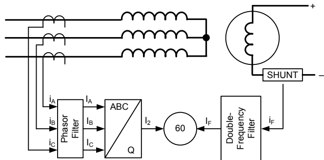
Fig. 15. Stator-rotor generator current balance scheme.
