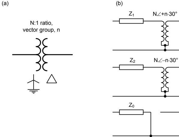
Fig. 4. Sequence networks for a grounded-wye / delta power transformer.
