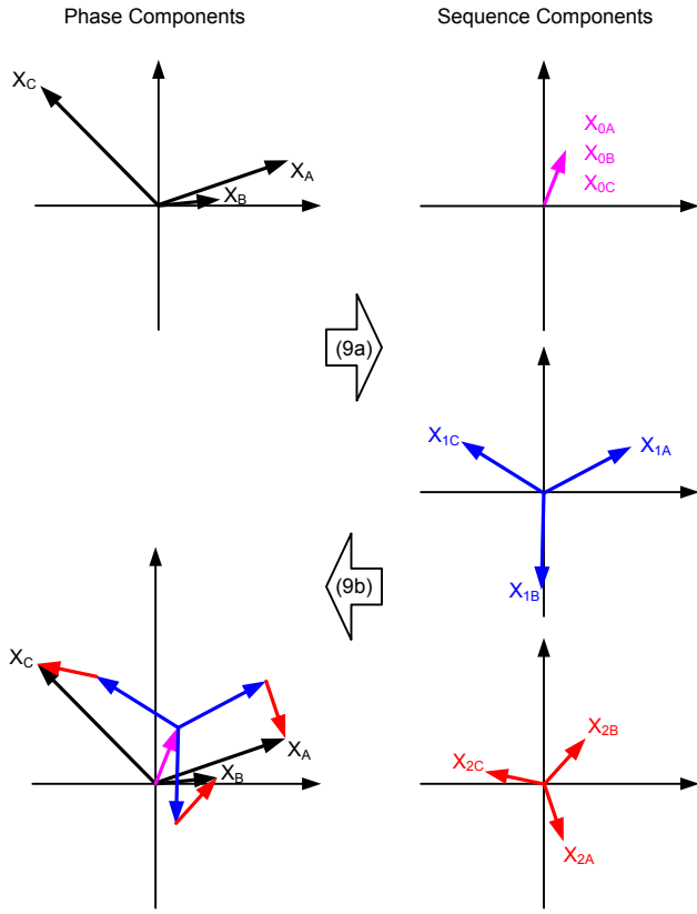
Fig. 1. A graphical example of converting phase components to sequence components and vice versa.
