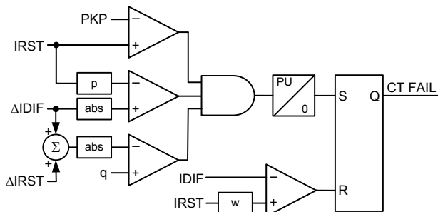
Fig. 20. Simplified CT failure logic in a differential protection application.
