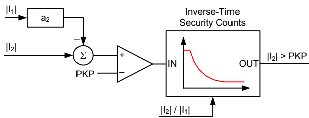
Fig. 24. The concept of positive-sequence restraining for system unbalances with inverse-time security counts.
