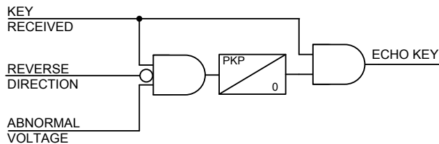
Fig. 26. Weak-infeed echo logic with increased security.
