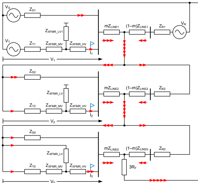
Fig. 32. Sequence network diagram for an AG fault for the system shown in Fig. 30 but with the WTG replaced by a conventional power source.
