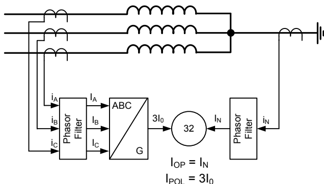
Fig. 14. REF protection using a directional operating principle.
