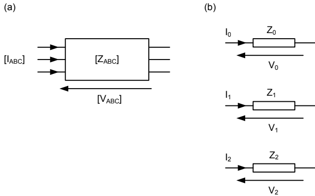
Fig. 2. Phase (a) and sequence (b) voltages, currents, and impedances.
