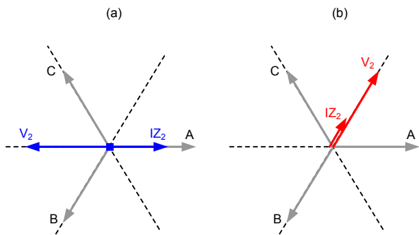
Fig. 28. Negative-sequence voltage and current for the forward AG fault (a) and reverse BG fault (b).
