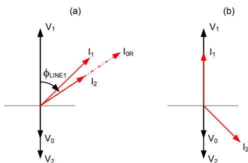
Fig. 38. Sequence components for the AG fault in the system of Fig. 35: traditional source as analyzed (a), IBR as recorded (b).
