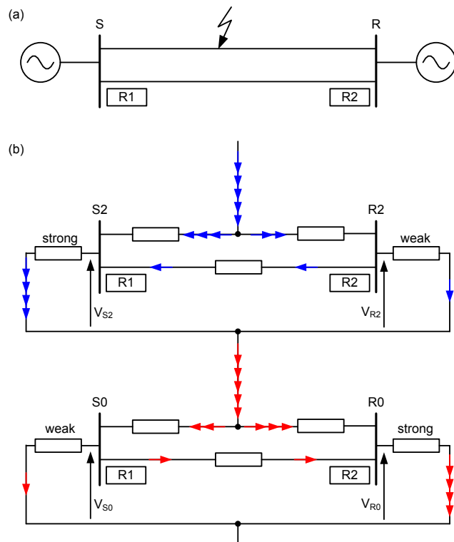
Fig. 25. A fault on a parallel path may cause the zero- and negative-sequence currents to flow in opposite directions: one-line diagram (a); zero- and negative-sequence networks connected for a single-phase fault (b).
