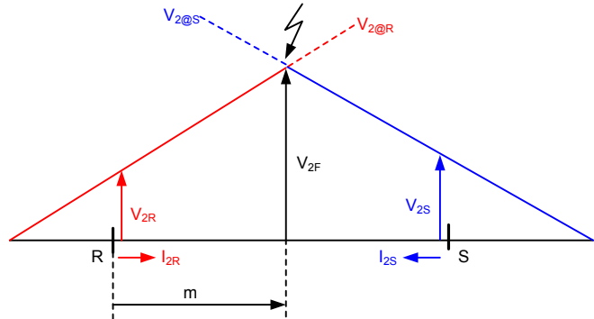
Fig. 21. Principle of the negative-sequence double-ended fault locator.
