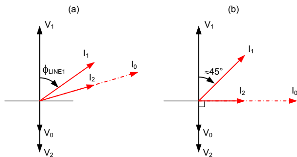
Fig. 33. Sequence components for the AG fault in the system of Fig. 30: traditional source as analyzed (a); Type 3 WTG source as recorded (b).
