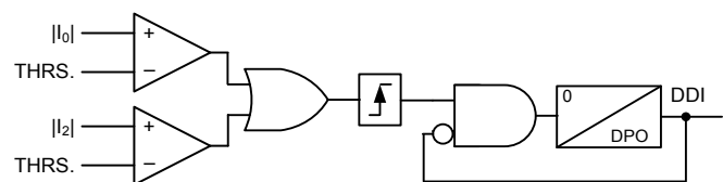
Fig. 18. Sample implementation of the disturbance detection logic using sequence currents.
