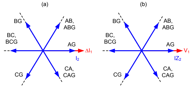
Fig. 12. Using the incremental positive-sequence current (a) and the positive-sequence voltage (b) to resolve single-phase and phase-to-phase faults (ABC phase rotation).
