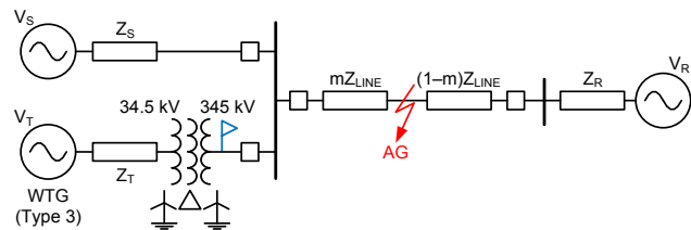
Fig. 30. One-line diagram of a power system with Type 3 WTGs.
