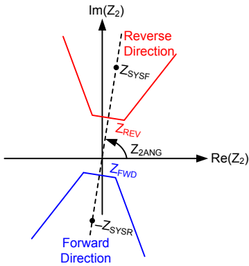
Fig. 9. Apparent-impedance-based implementation of the negative-sequence directional element (32Q).
