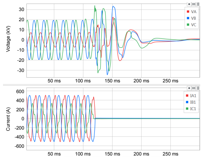
Fig. 36. Phase voltages and currents recorded by the relay at the IBR source.
