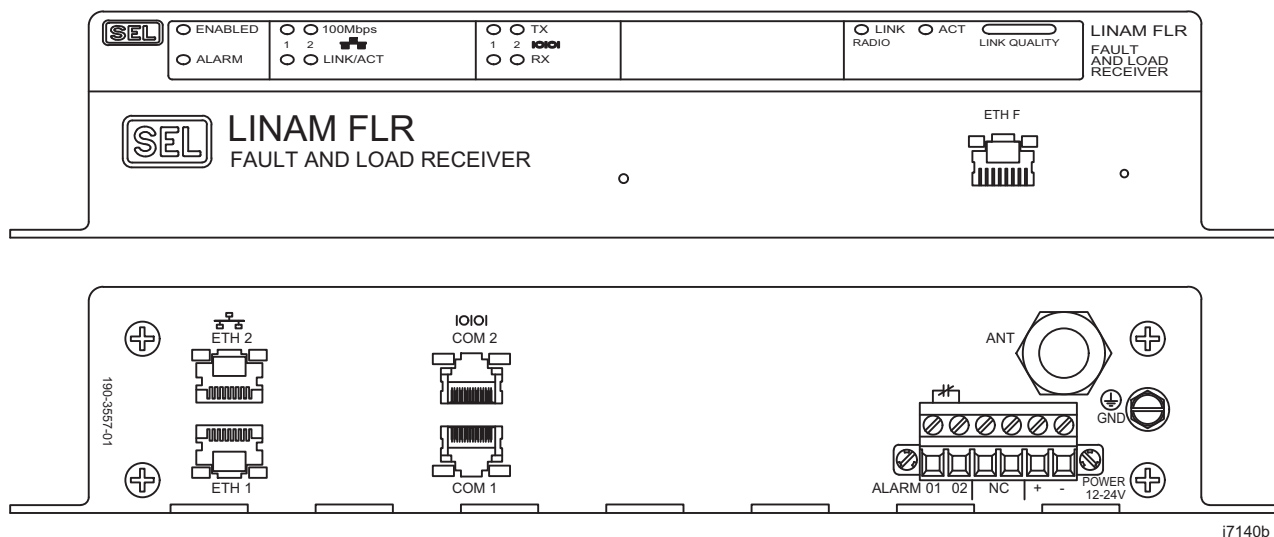
Figure 11 FLR Diagram
