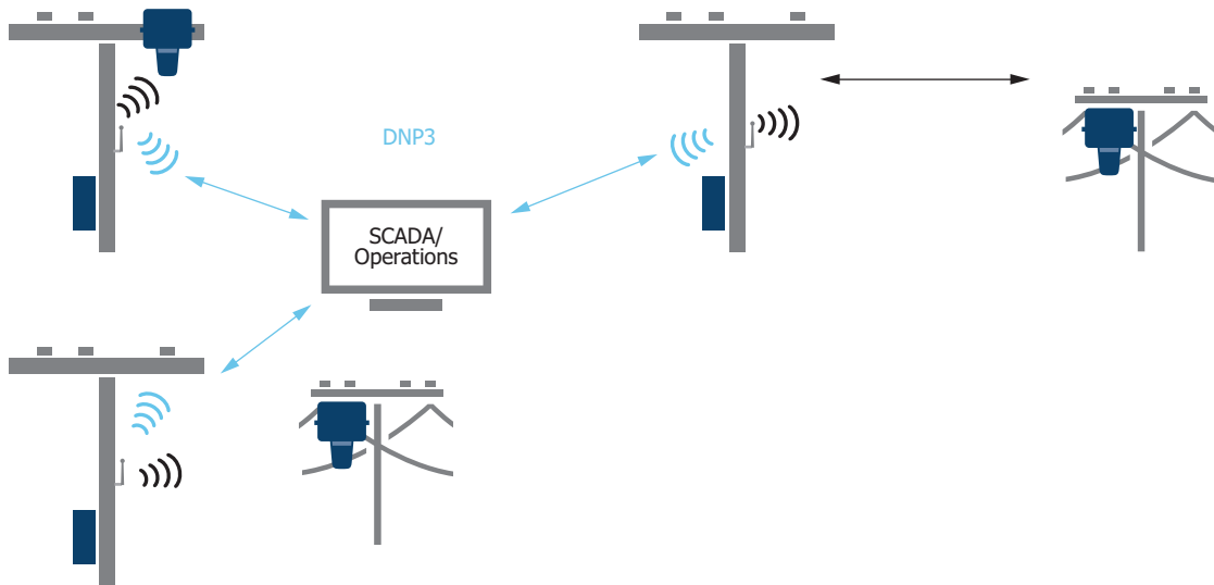
Figure 4 Network Diagram
