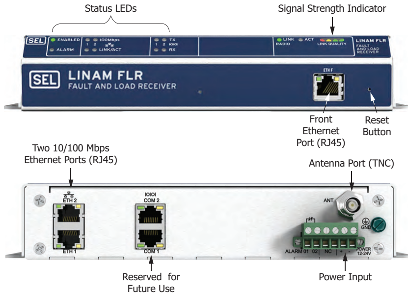
Figure 3 FLR Device Overview
