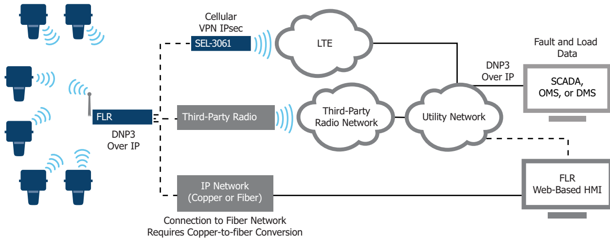
Figure 1 Functional Diagram
