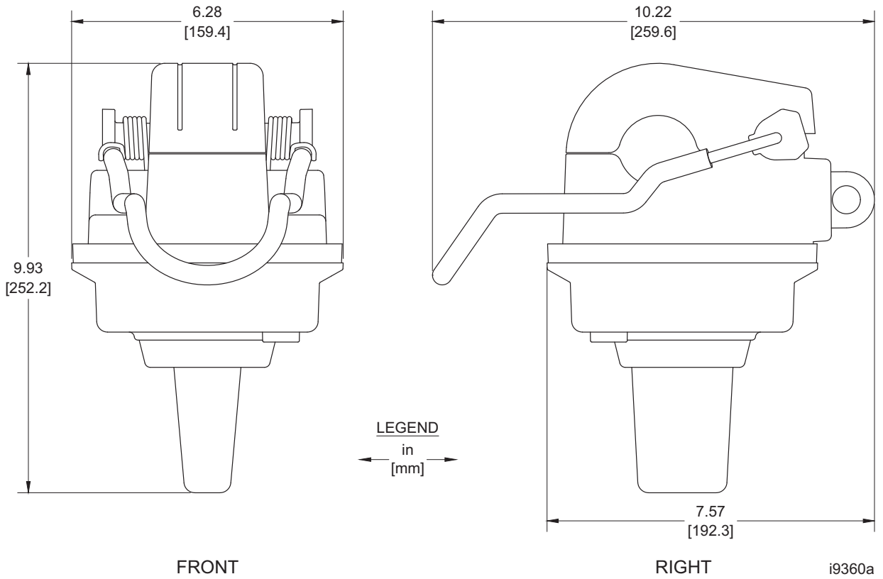
Figure 12 FLT Dimensions
