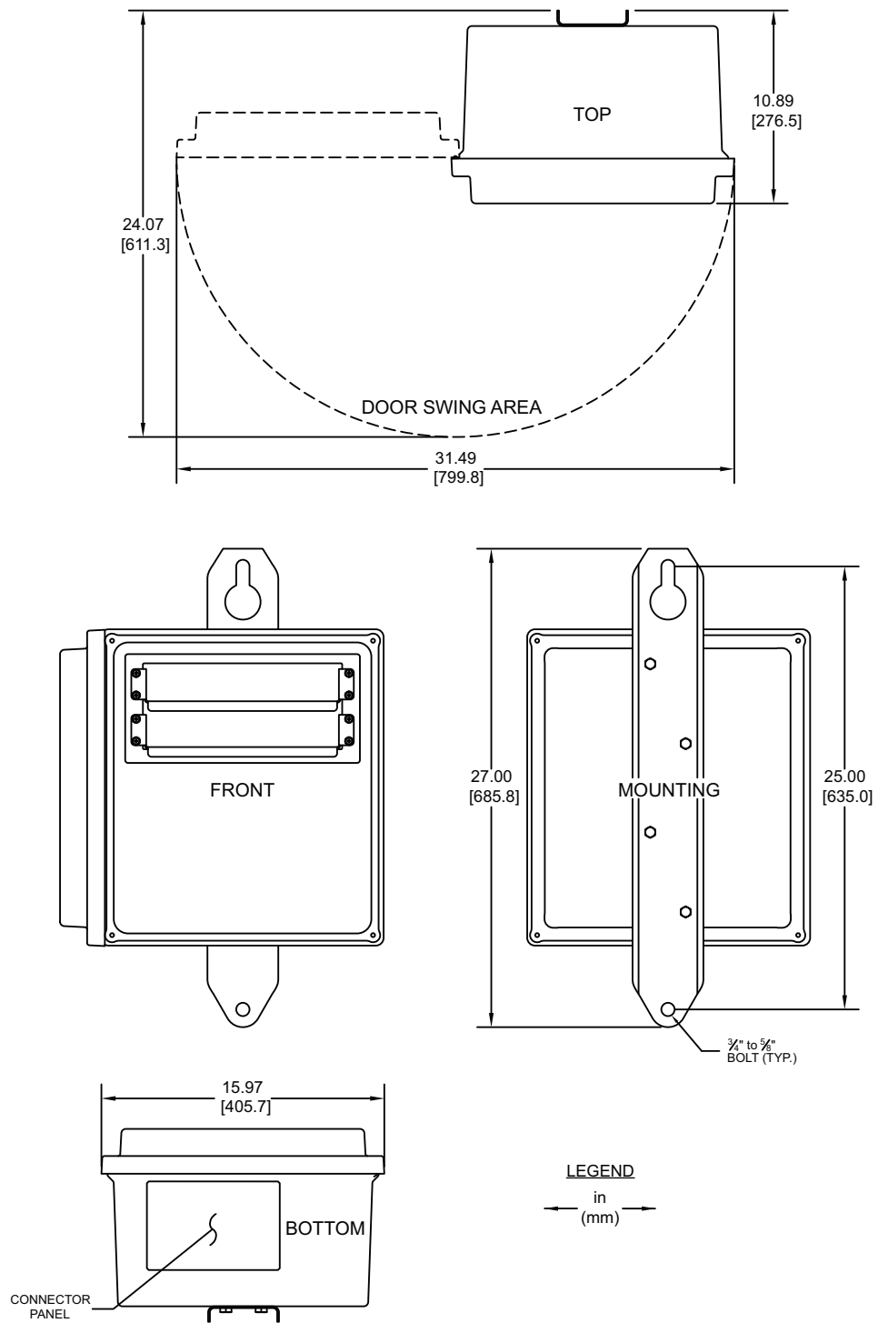
Figure 14 FLR Enclosure Dimensions
