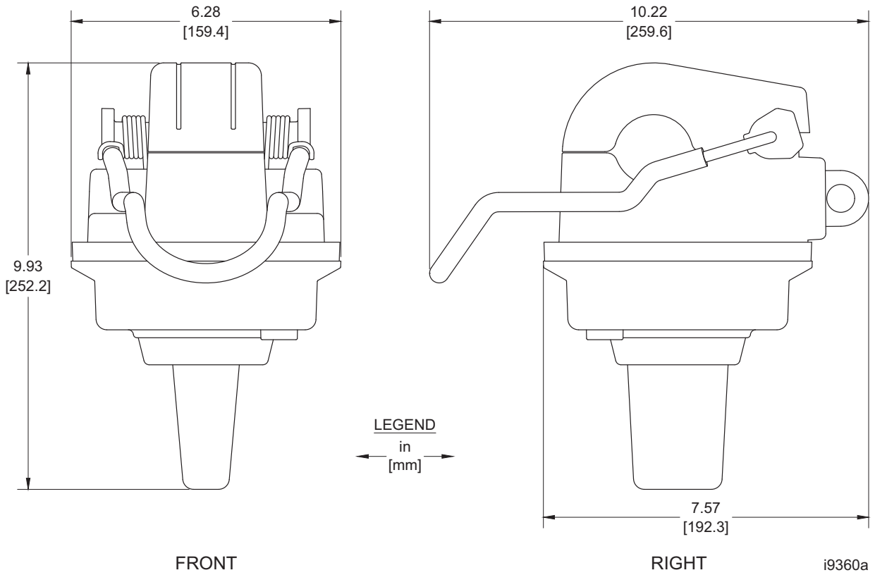
Figure 12 FLT Dimensions
