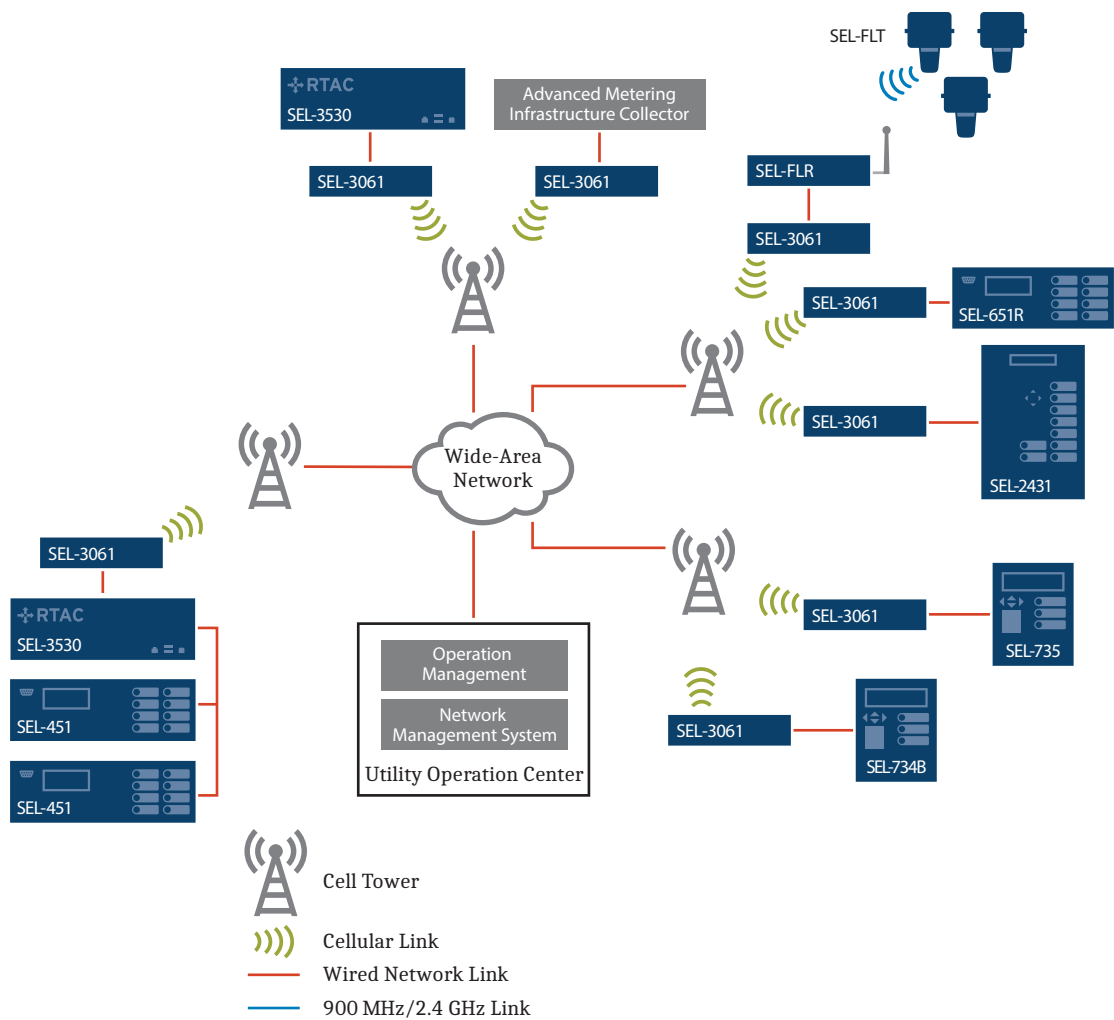
Figure 2 Application Overview
