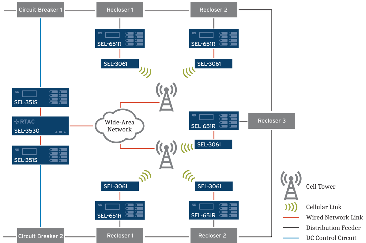
Figure 4 Distribution Automation
