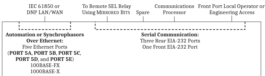
Figure 17 System Functional Overview
