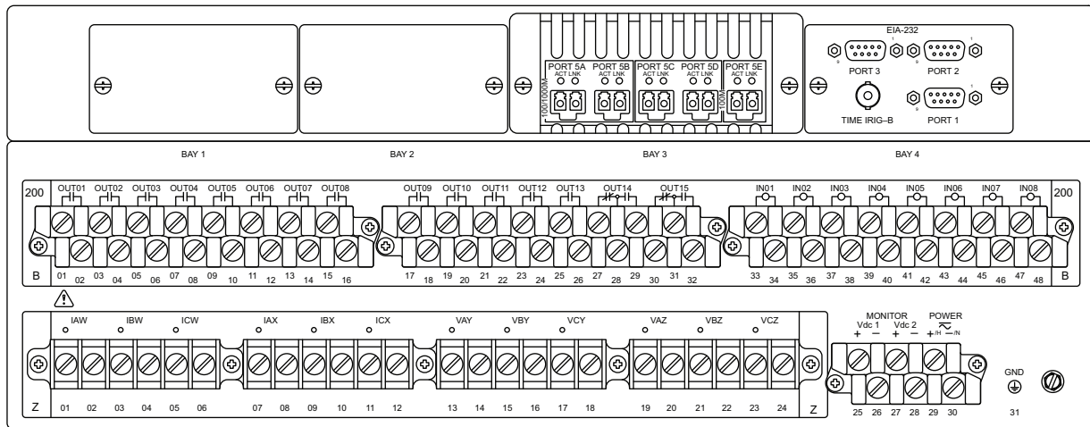
Figure 23 SEL-451-6 SV Publisher, 4U Rear Panel
