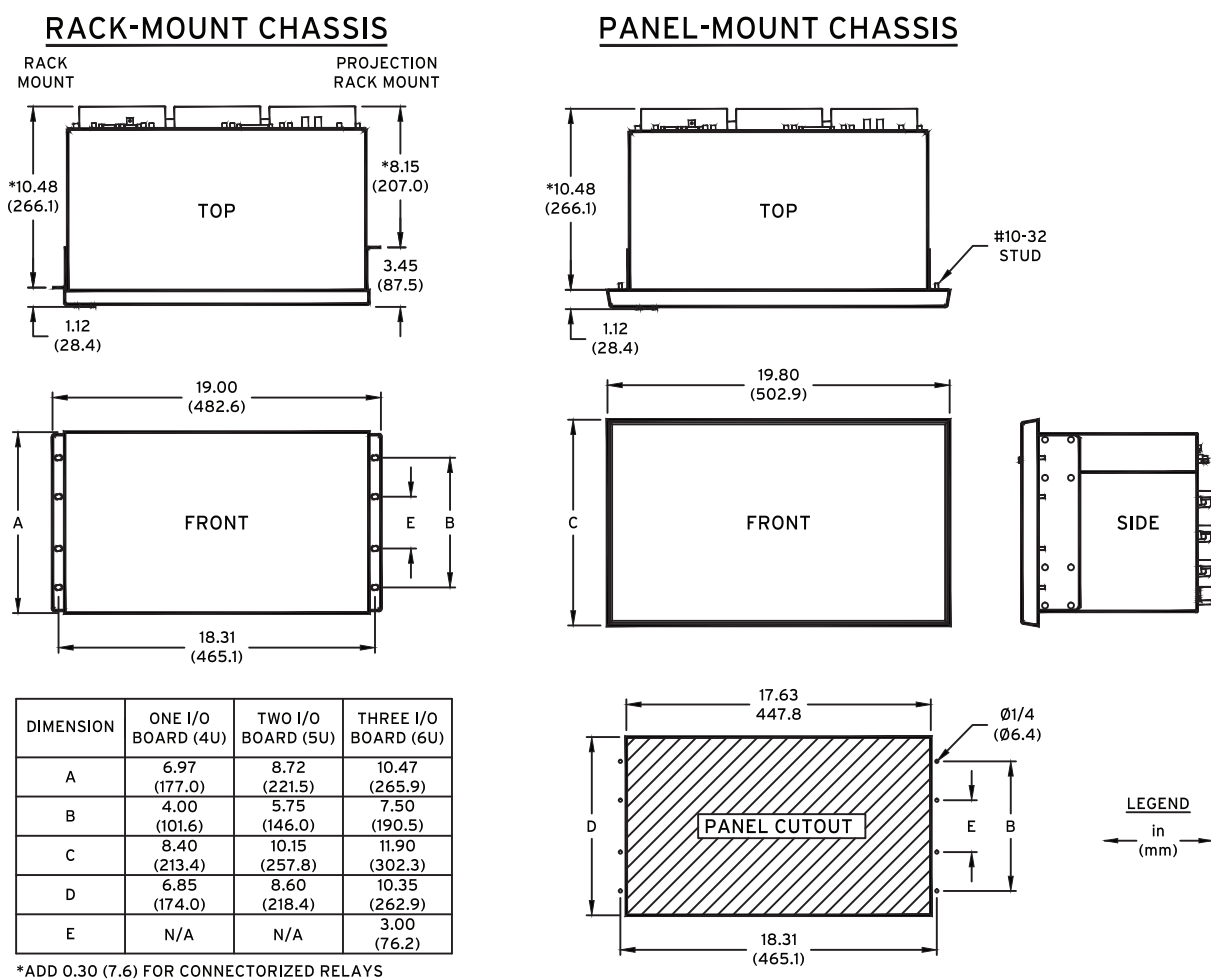
Figure 24 Dimensions for Rack- and Panel-Mount Models
