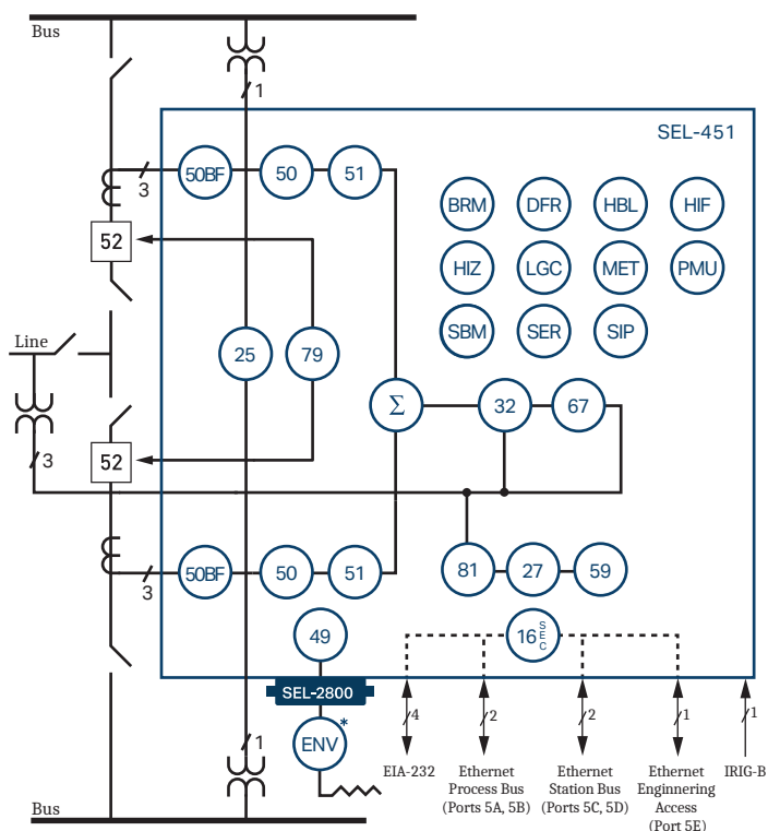
Figure 1 SEL-451-6 SV Subscriber or TiDL Functional Overview
