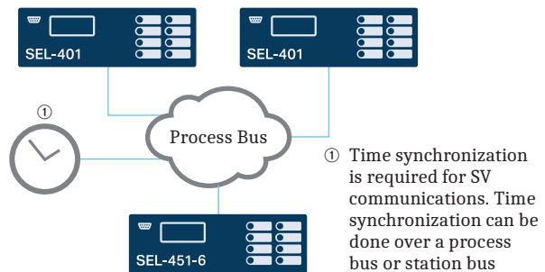
Figure 3 SV Network
