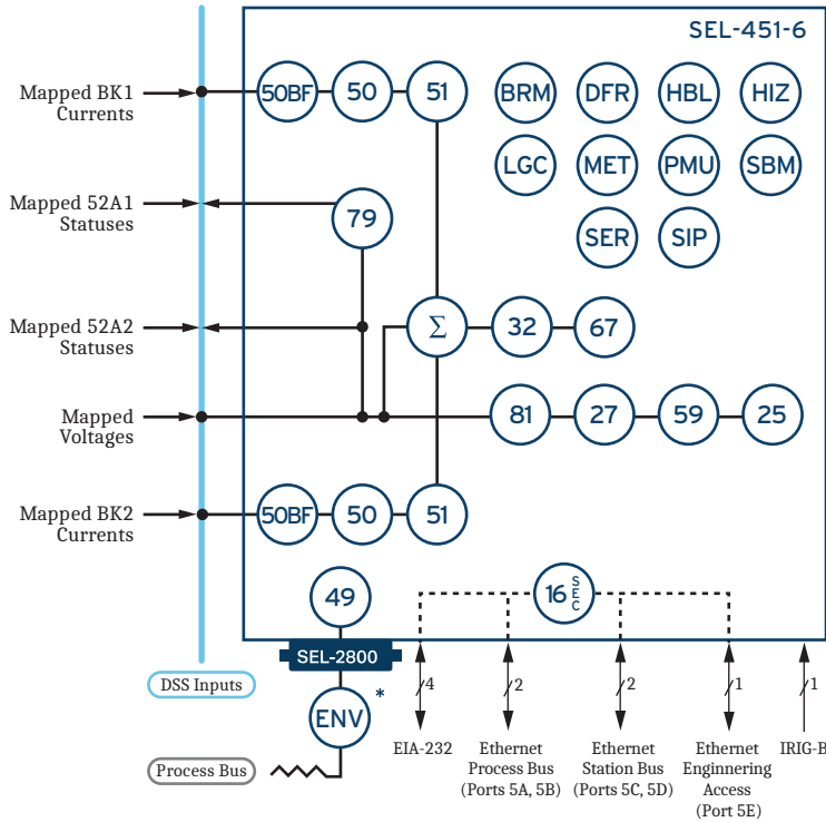
Figure 1 SEL-451-6 SV Subscriber or TiDL Functional Overview
