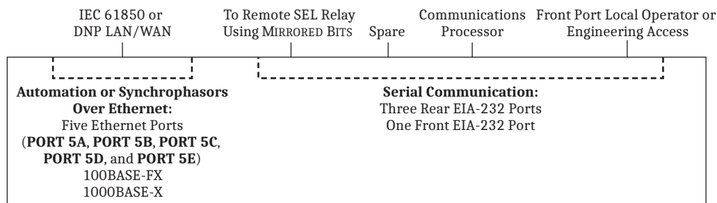
Figure 17 System Functional Overview
