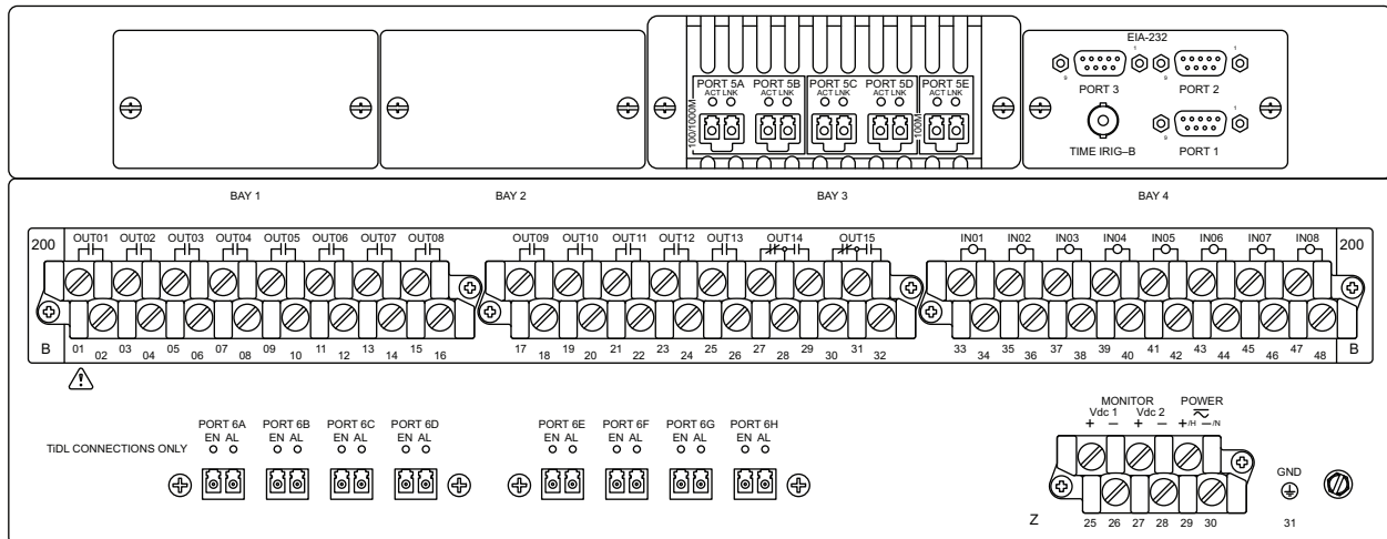
Figure 24 SEL-451-6 TiDL Relay, 4U Rear Panel
