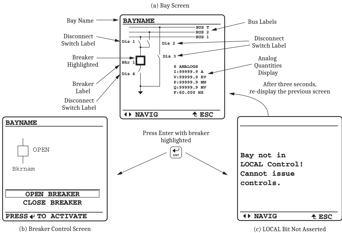
Figure 14 Screens for Circuit Breaker Selection
