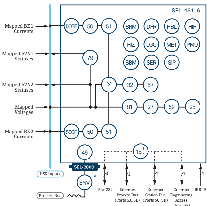
Figure 2 SEL-451-6 SV Publisher Functional Overview
