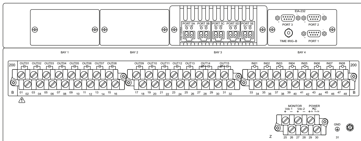
Figure 22 SEL-451-6 SV Subscriber, Rear Panel
