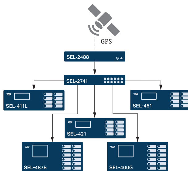
Figure 18 Example PTP Network
