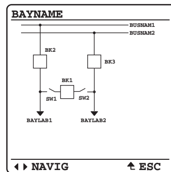
Figure 10 Breaker-and-a-Half
