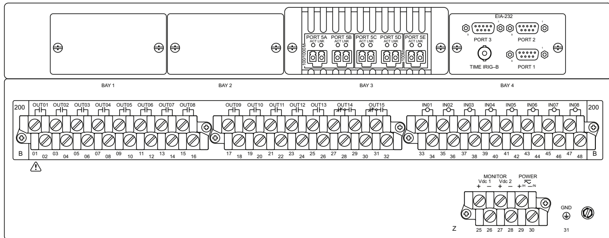
Figure 22 SEL-451-6 SV Subscriber, Rear Panel
