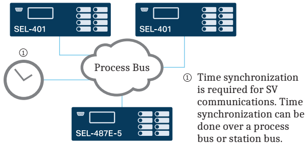
Figure 3 SV Network
