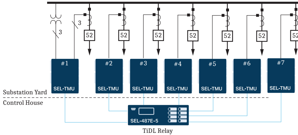
Figure 14 Seven Terminal Feeder Application (TiDL)
