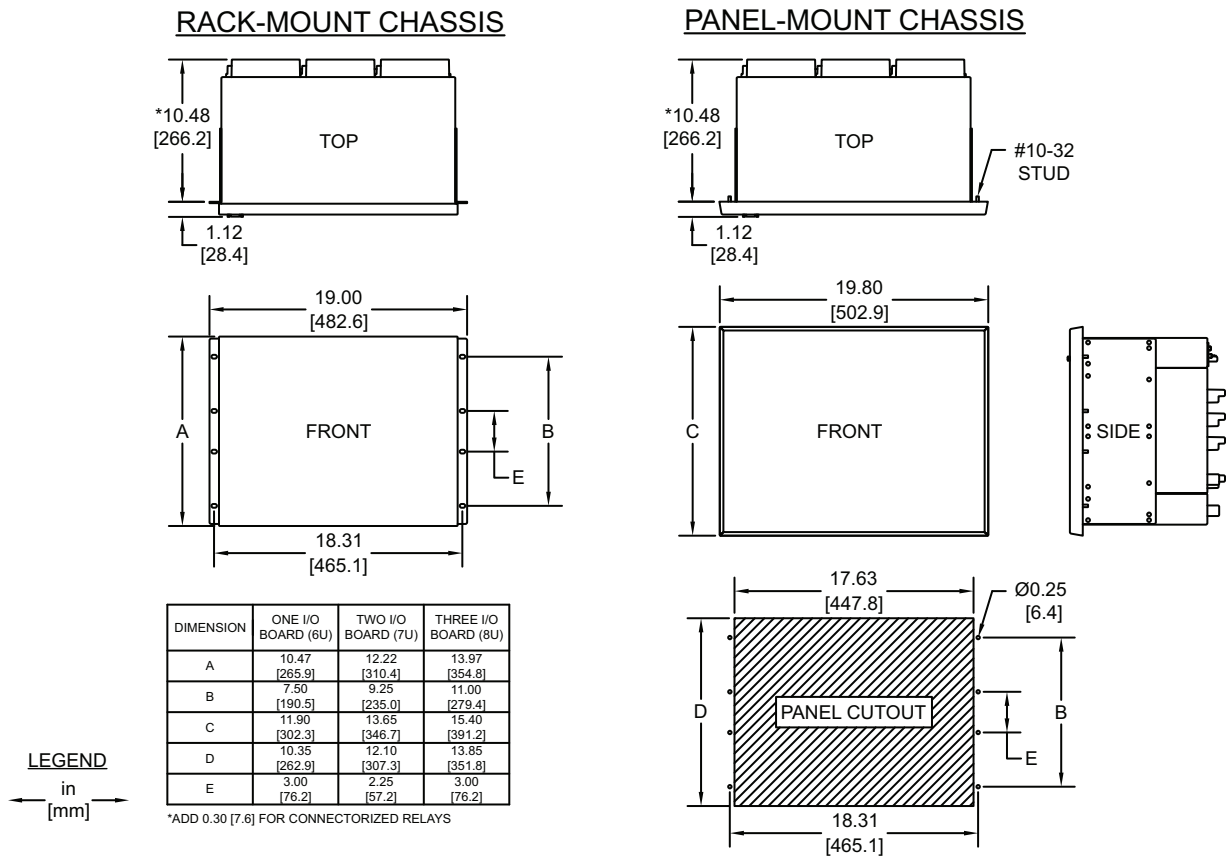
Figure 36 SEL-487E Chassis Dimensions With Dual AC Input Cards
