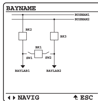
Figure 17 Breaker-and-a-Half
