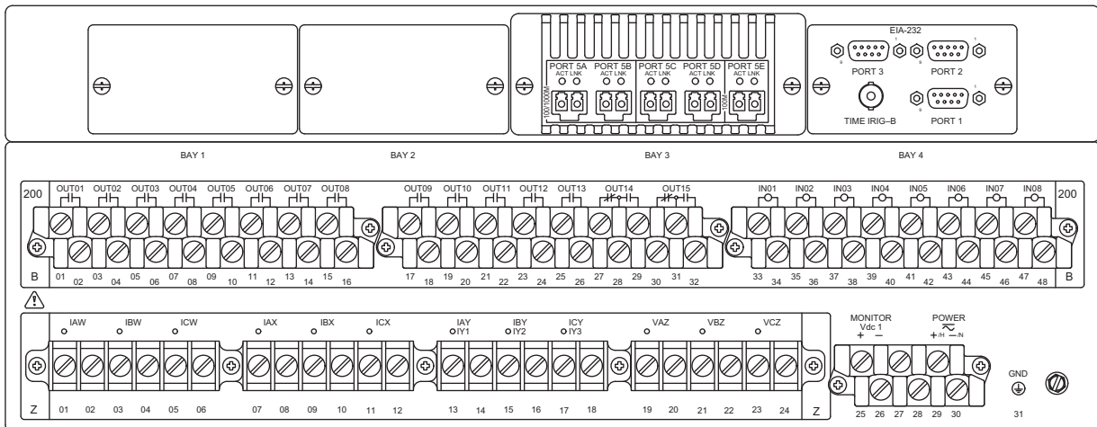
Figure 34 Single AC Input Card Rear Panel With Fixed Terminal Blocks (4U)
