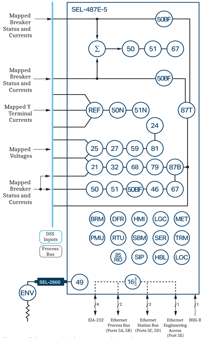
Figure 2 SEL-487E-5 SV Subscriber or TiDL Relay Functional Overview
