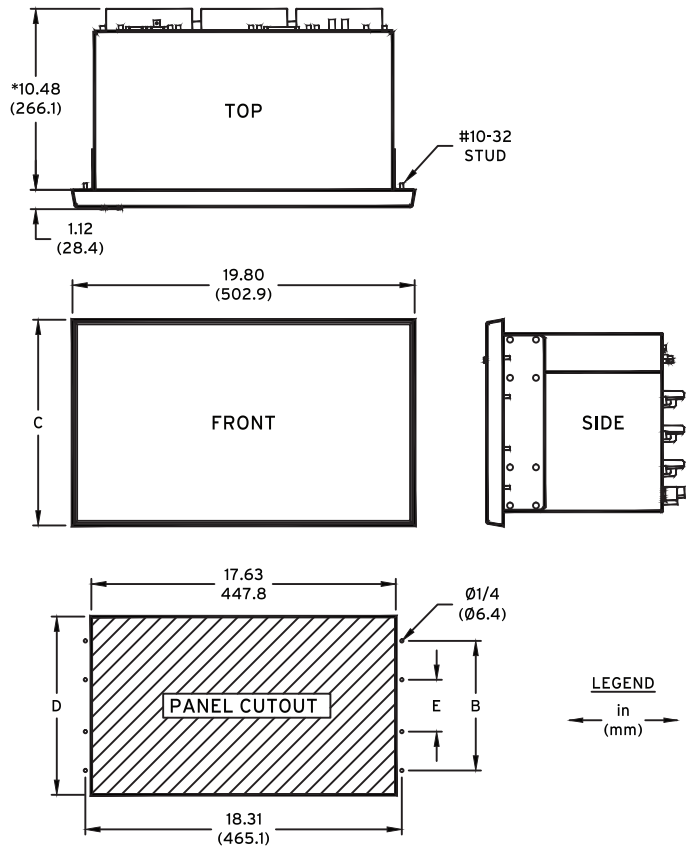
Figure 35 SEL-487E Chassis Dimensions for TiDL Relays, SV Subscribers, or Relays With a Single AC Input Card
