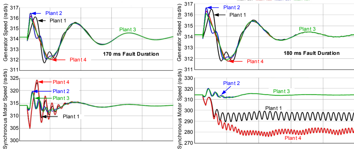
Fig. 10 Determination of Fault Clearing Time
