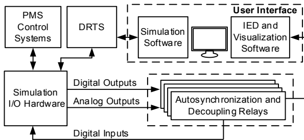
Fig. 7 Closed-Loop Simulation Setup
