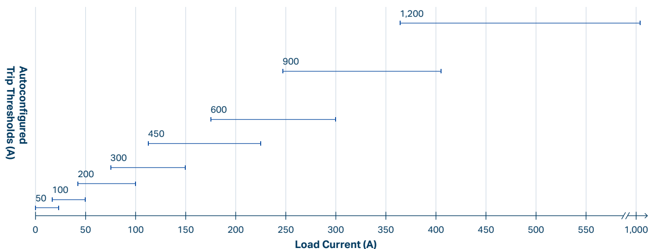
Figure 1: Autoranging Graph Used by AR-URD to Configure Trip Threshold
