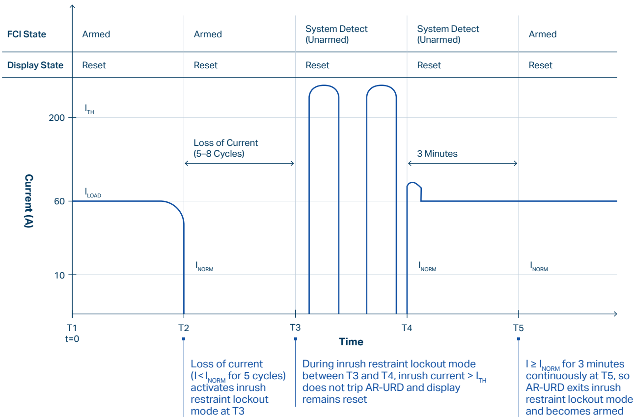
Figure 2: Response of AR-URD to Inrush Currents Falsely Appearing as Fault Currents
