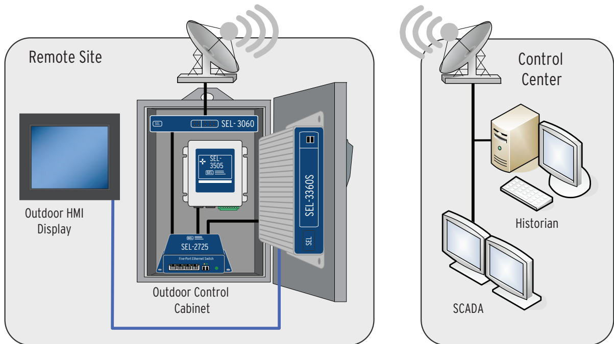
Figure 1 SEL-3360-2 in Monitoring and Control Applications
