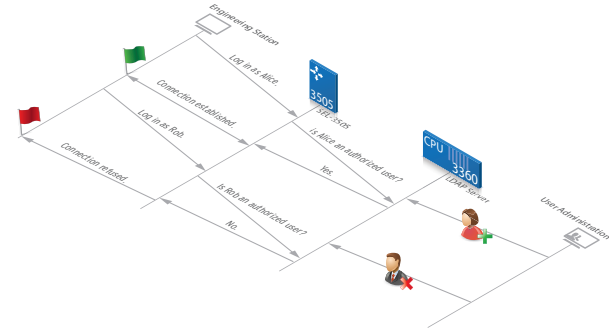
Figure 4 SEL-3360-2 as Remote Read-Only Domain Controller Performing Central Authentication Using LDAP
