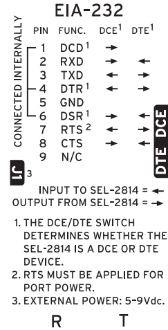
Figure 6 SEL-2814 Signal Flow
