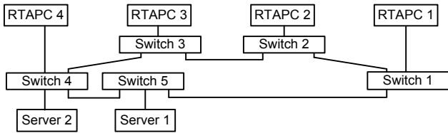
Figure 2. Schematic Diagram of Cyber Network in a Microgrid
