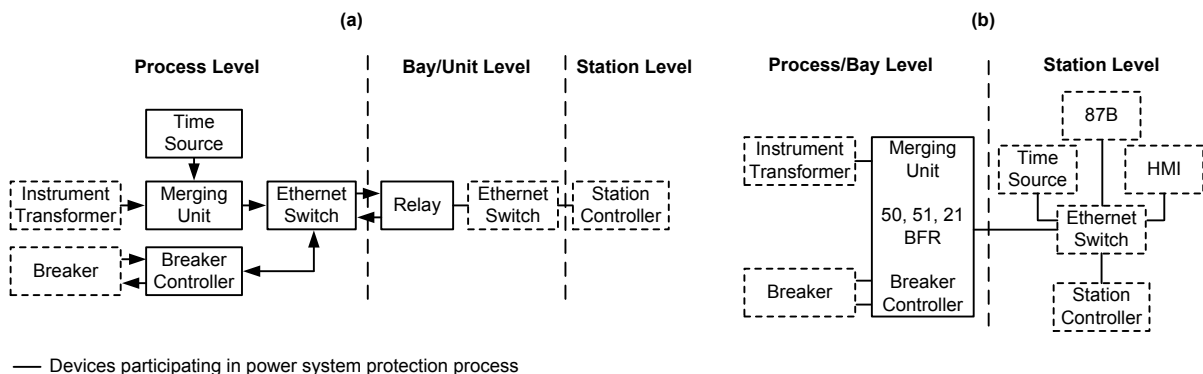
Figure 2: (a) Simplified substation block diagram indicating core devices and their traditional associated logical levels and (b) a modern, full-featured merging unit installation with local protection and control
