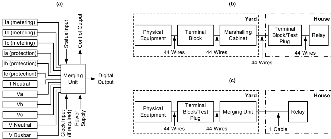
Figure 1: (a) Merging unit concept per IEC 60044-8 with status and controls added, (b) traditional wiring approach with relays in the control house, and (c) simplified diagram showing cable reduction potential with Ethernet-based merging unit technology
