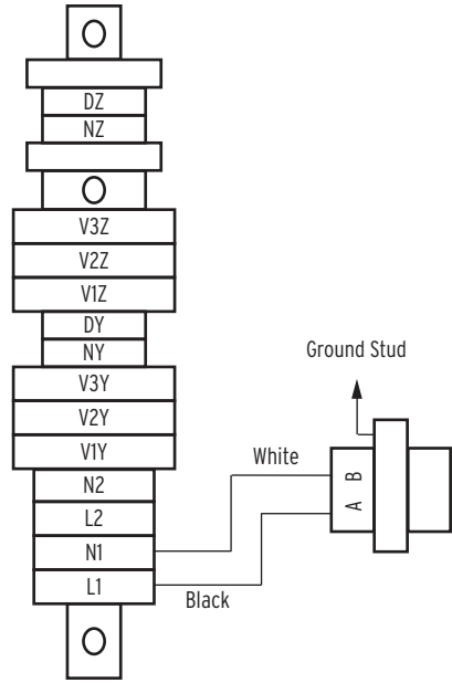
Wiring between fuse block and control module not shown.
