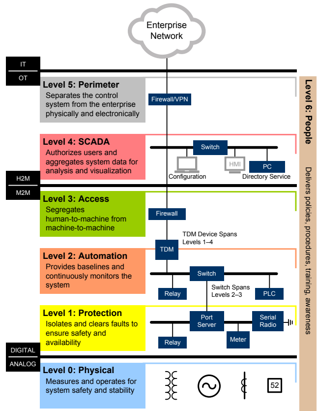
Fig. 3. Defense-In-Depth Model
