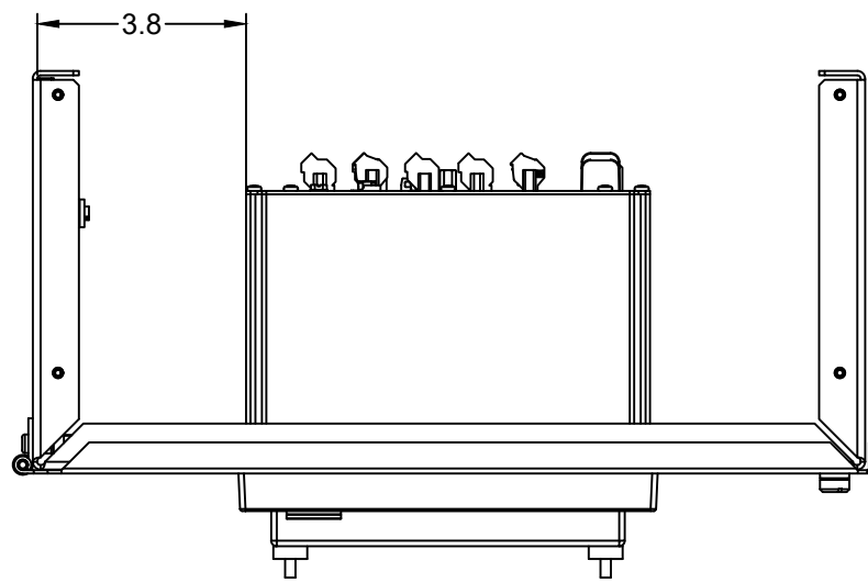
TOP VIEW (ALUMINUM SWING PANEL AND CHASSIS)
