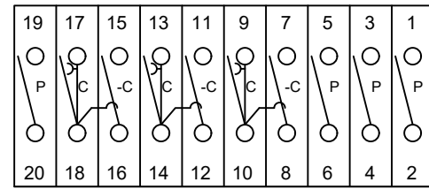
TEST SWITCH CONFIGURATION (REAR VIEW)
