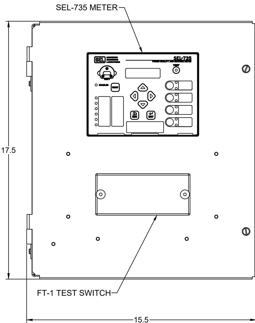
FRONT VIEW (ALUMINUM SWING PANEL AND CHASSIS)
