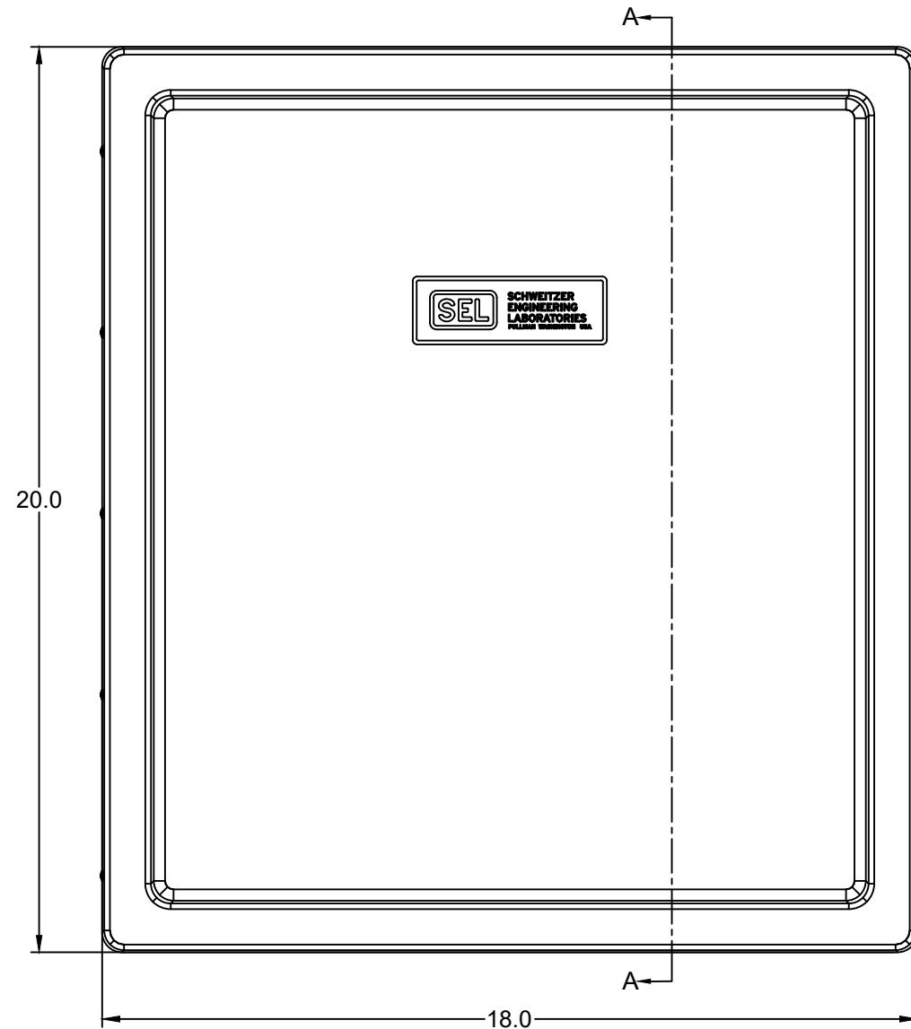
FRONT VIEW (UL TYPE 4X FIBERGLASS ENCLOSURE)
