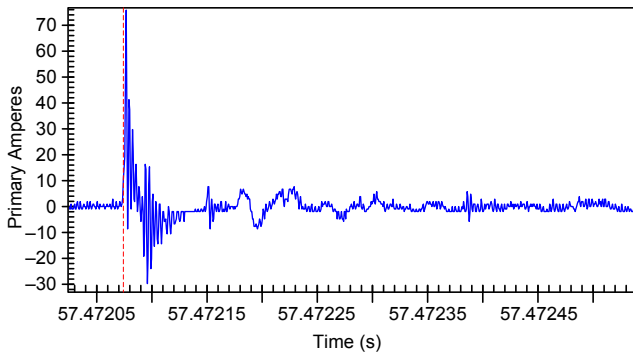
Fig. 10. Current TWs for a C-phase-to-ground fault used for fault locating.
