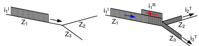
Fig. 1. Current TW passing through a junction point.
