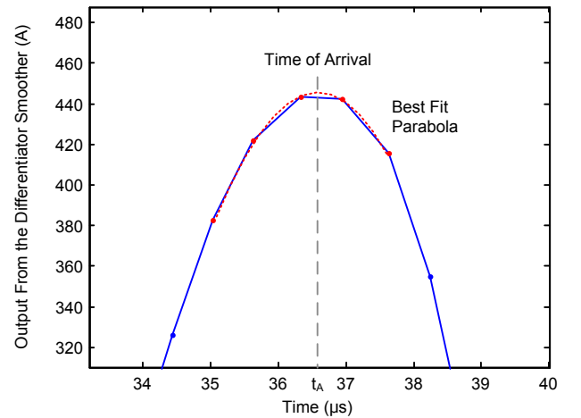
Fig. 5. Accurate time-stamping of the TW using the best-fit parabola.
