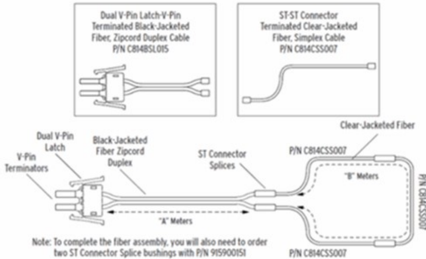
Figure 1 - Bare-Fiber Sensor Assembly with two additional ST Splice Connectors
