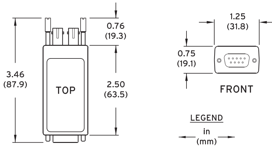
Figure 14 SEL-3405 Dimensions
