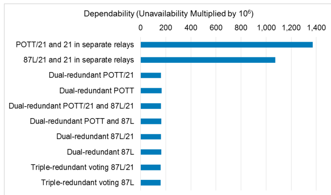
Fig. 37. Fault tree analysis results: Line protection dependability comparison.
