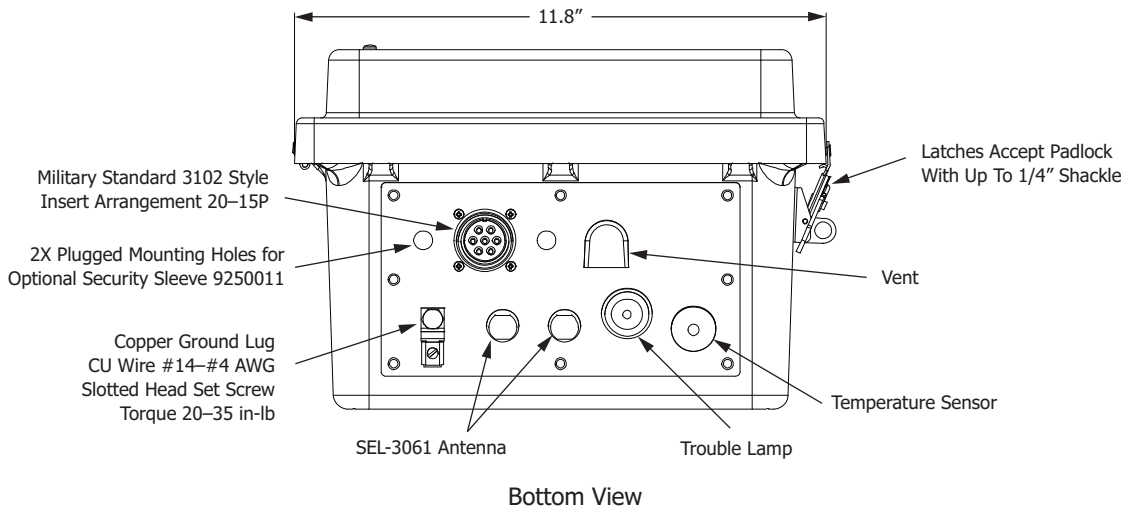
Figure 2.4 Bottom View of Connectorized Compact Enclosure
