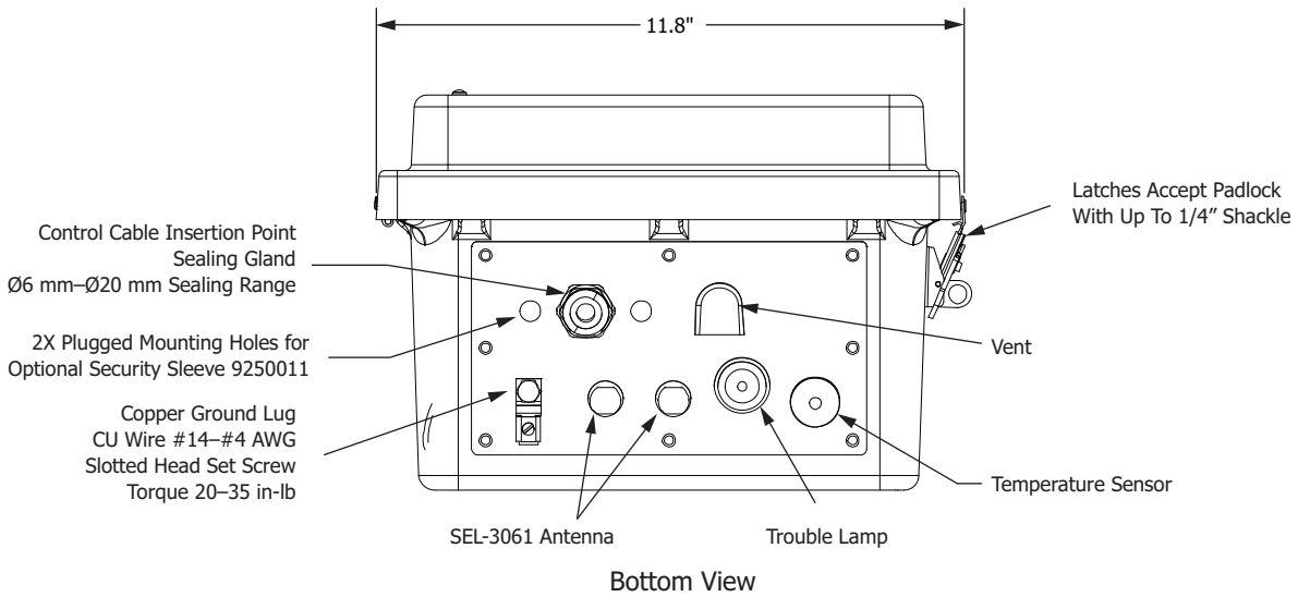
Figure 2.5 Bottom View of Terminal Block Enclosure
