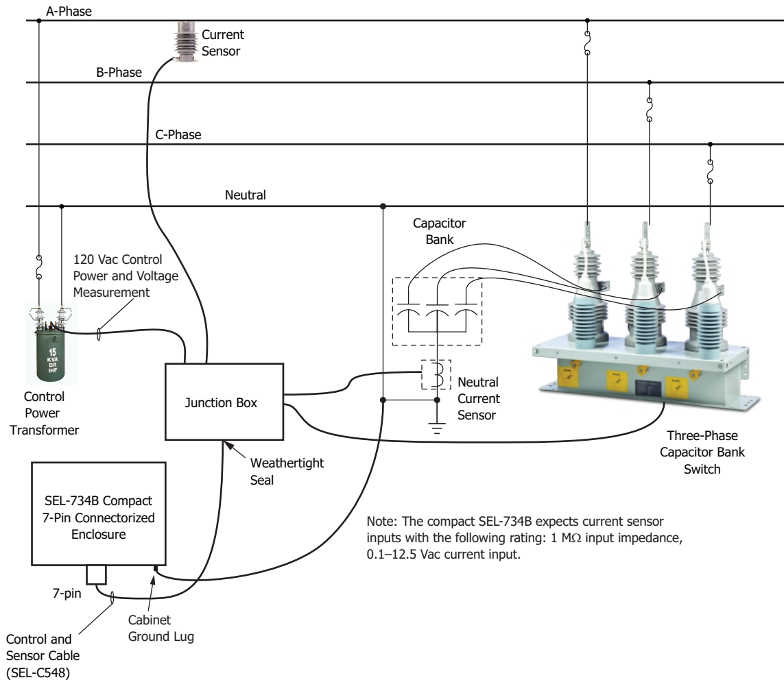
Figure C.6 Compact 7-Pin Connectorized Enclosure
