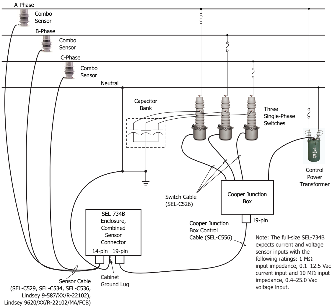
Figure C.2 Full-Size Enclosure With Combined Sensor Connector (Installed With Cooper Junction Box)
