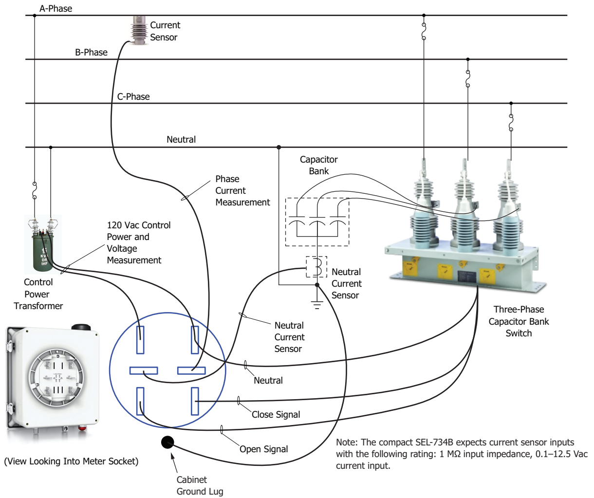
Figure C.8 Compact 6-Jaw Option A Socket-Based Enclosure Connection Diagram
