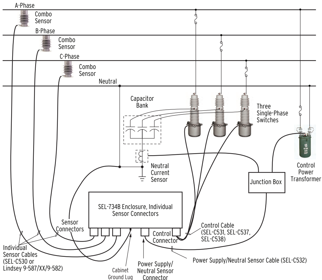
Figure C.3 Full-Size Enclosure With Individual Sensor Connectors (Installed With a Generic Neutral Current Sensor)
