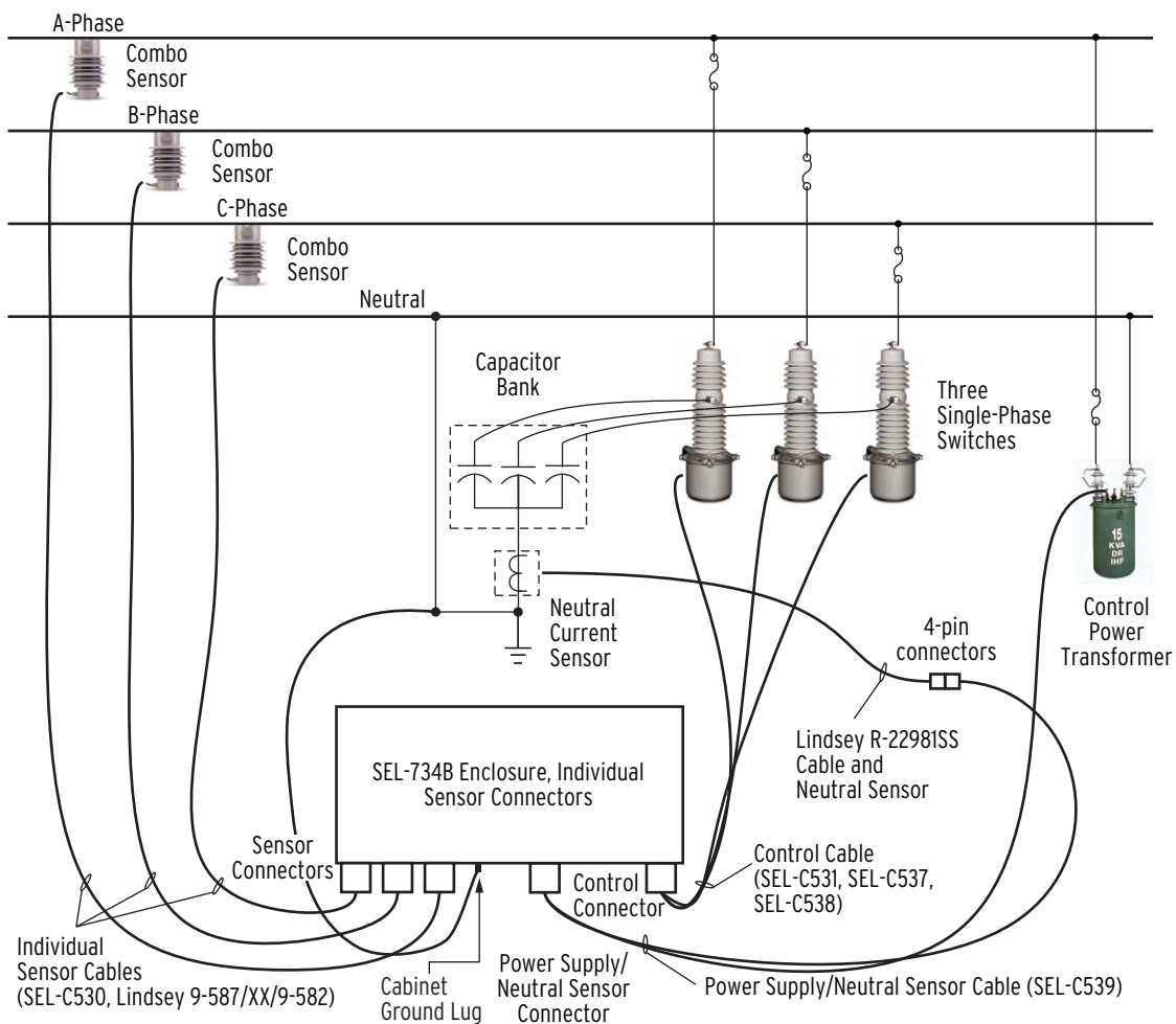
Figure C.4 Full-Size Enclosure With Individual Sensor Connectors (Installed With a Lindsey Neutral Current Sensor)
