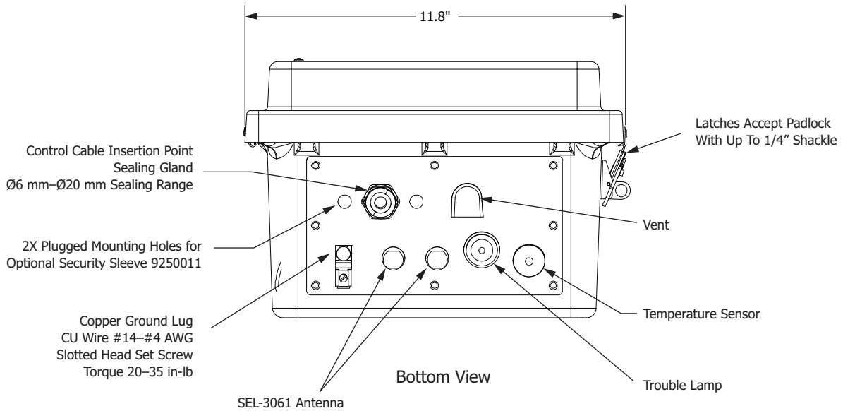
Figure 2.5 Bottom View of Terminal Block Enclosure
