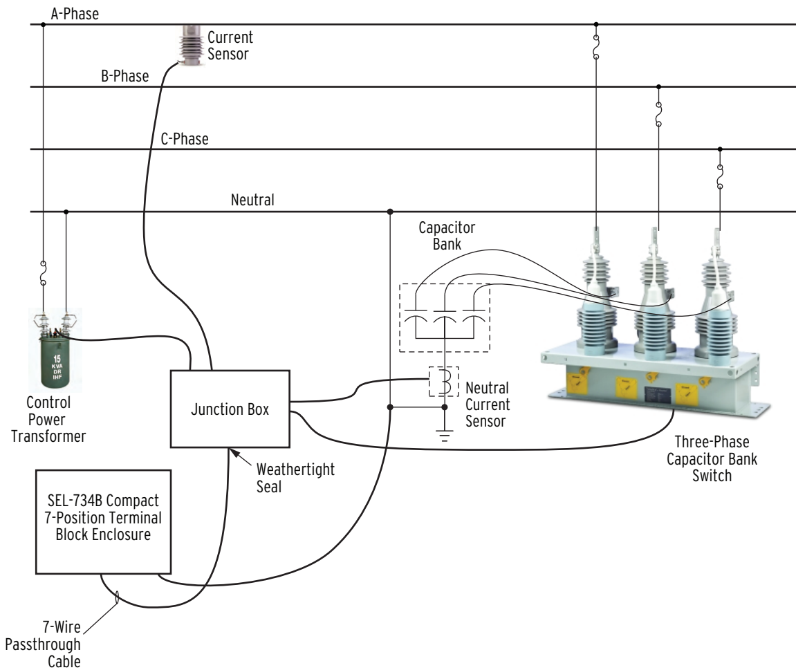
Figure C.7 Compact 7-Position Terminal Block Enclosure
