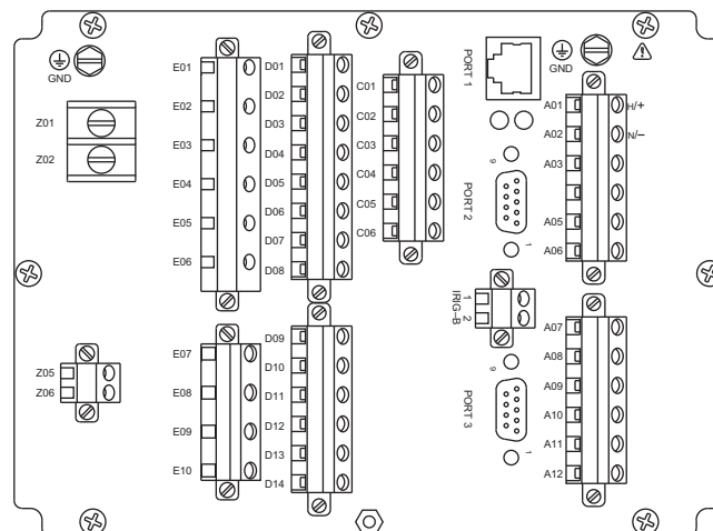
Figure 1.3 Top Label and Rear Panel
