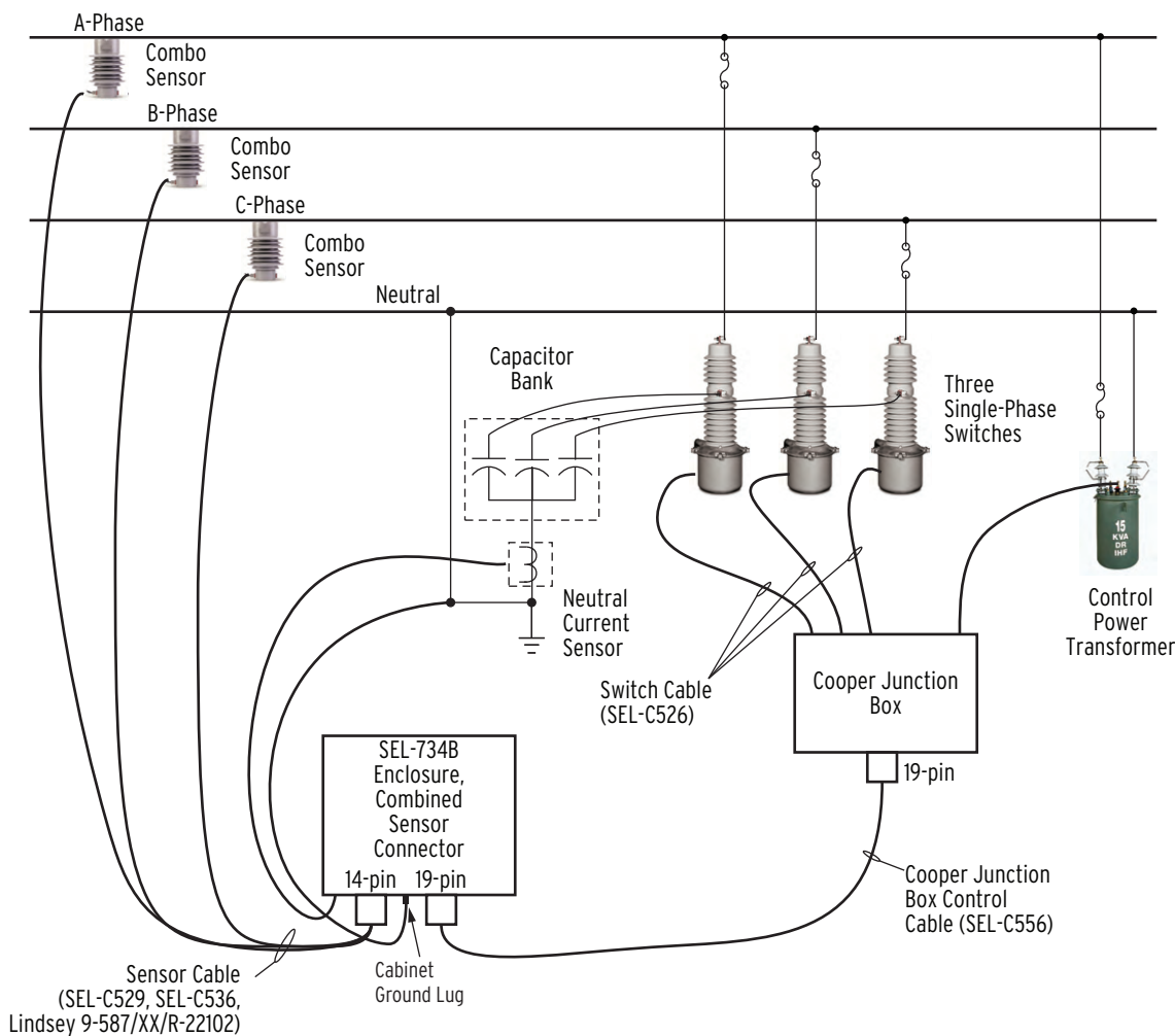
Figure C.2 Full-Size Enclosure With Combined Sensor Connector (Installed With Cooper Junction Box and Separate Neutral Sensor Cable)
