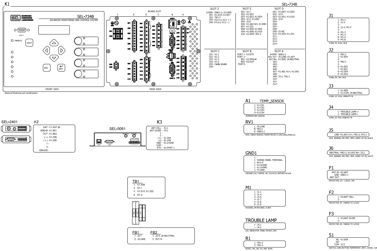
Figure E.4 Compact 6-Jaw Option A Socket-Based Enclosure Point-to-Point Wiring Diagram
