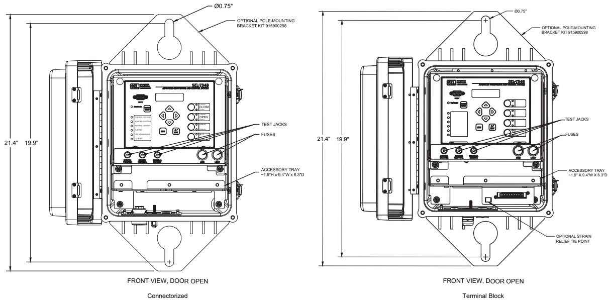
Figure 3.3 Compact 7-Pin Enclosure Mounting Dimensions
