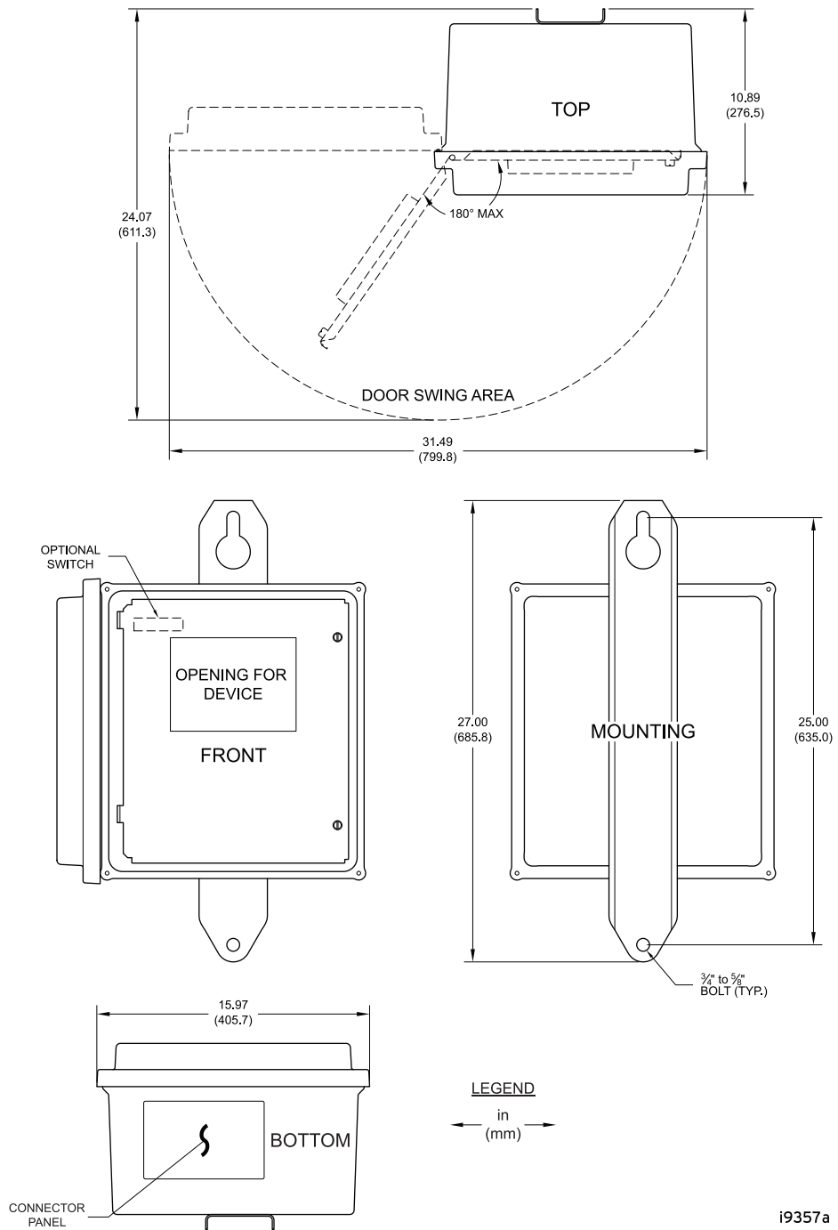
Figure 3.2 Full-Size Enclosure Mounting Dimensions
