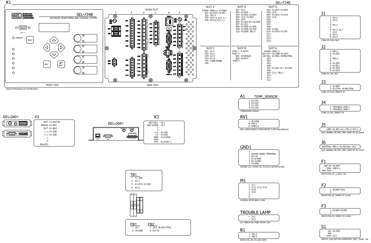
Figure E.2 Compact 4-Jaw Socket-Based Enclosure Point-to-Point Wiring Diagram
