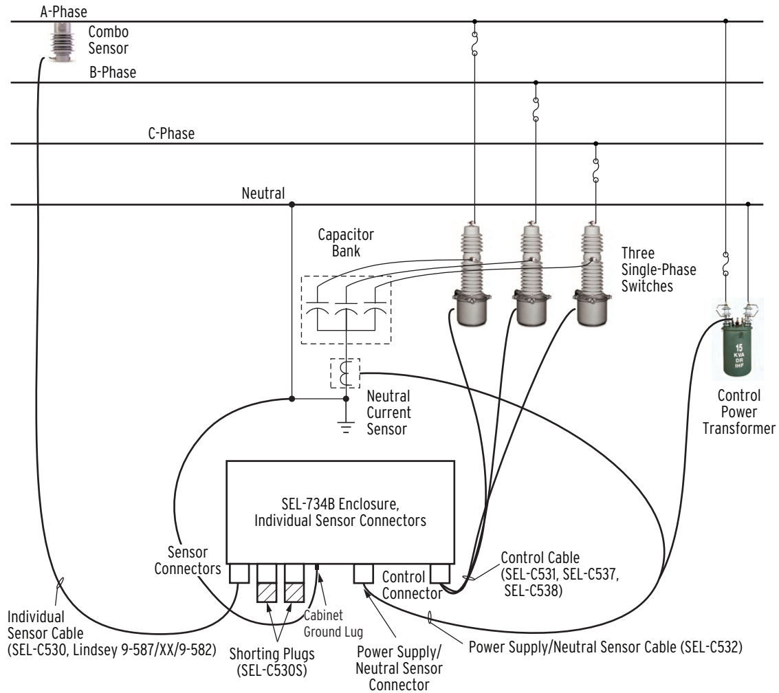
Figure C.5 Full-Size Enclosure With Individual Sensor Connectors (Installed With a Single Sensor and Generic Neutral Current Sensor)
