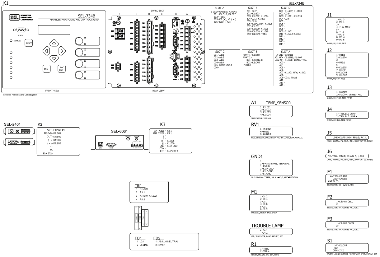
Figure E.6 Compact 6-Jaw Option B Socket-Based Enclosure Point-to-Point Wiring Diagram
