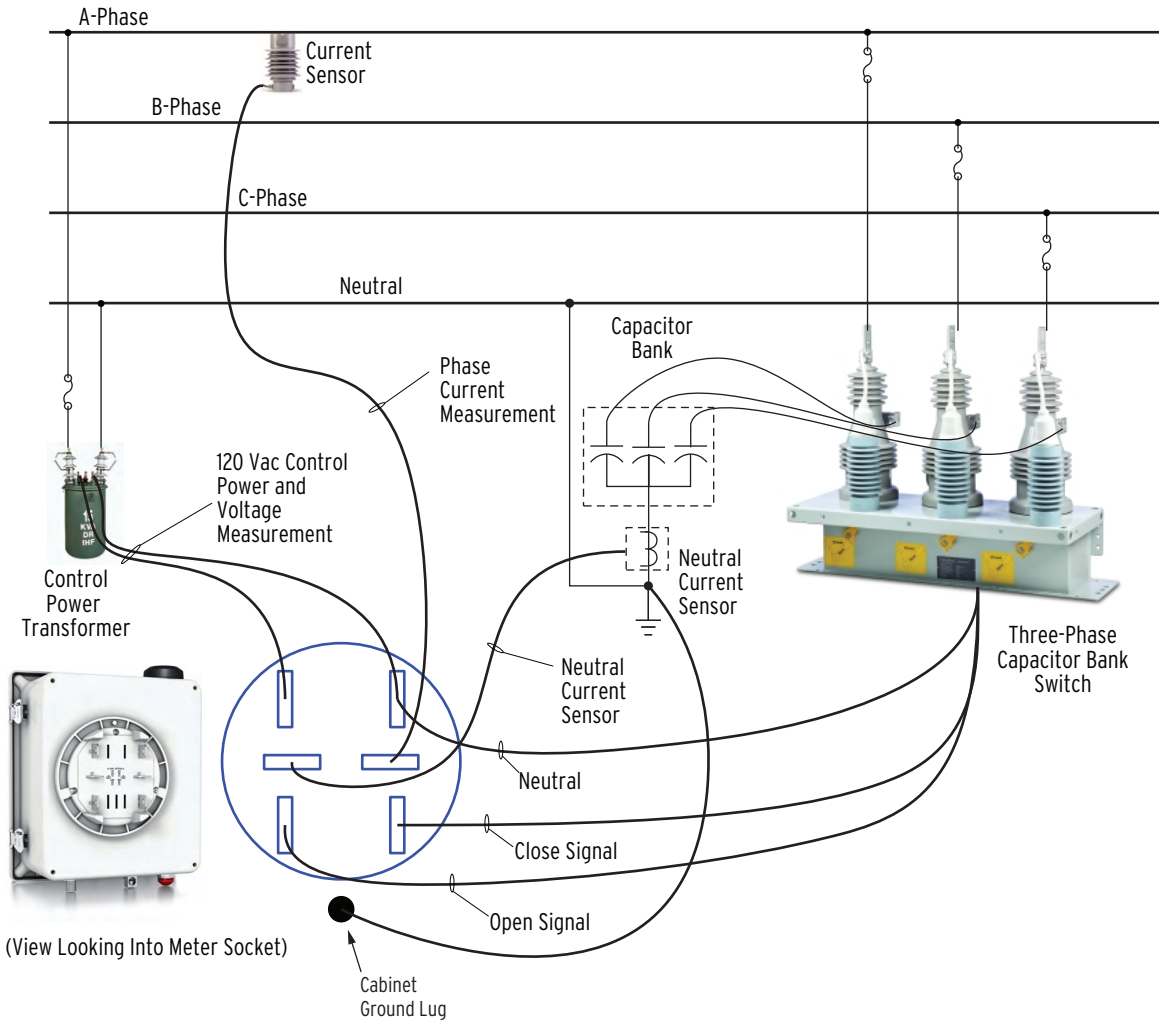
Figure C.8 Compact 6-Jaw Option A Socket-Based Enclosure Connection Diagram
