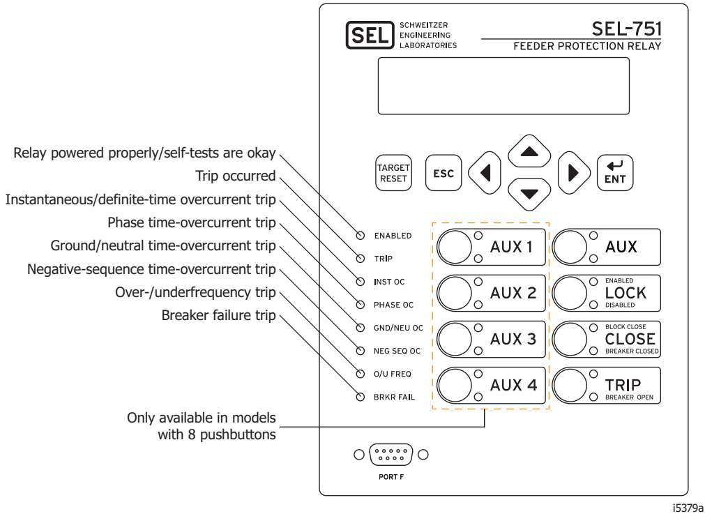
Figure 35 Front Panel With Default Configurable Labels
