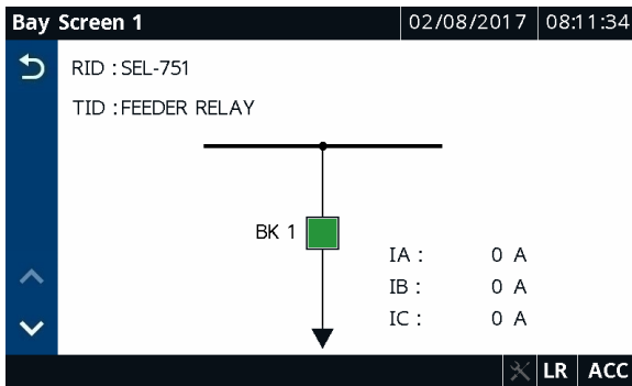
Figure 19 Default Bay Screen
