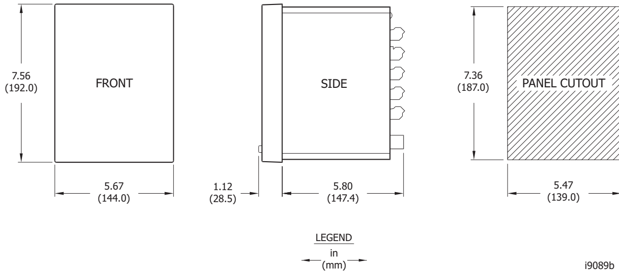
Figure 33 SEL-751 Dimensions for Rack- and Panel-Mount Models
