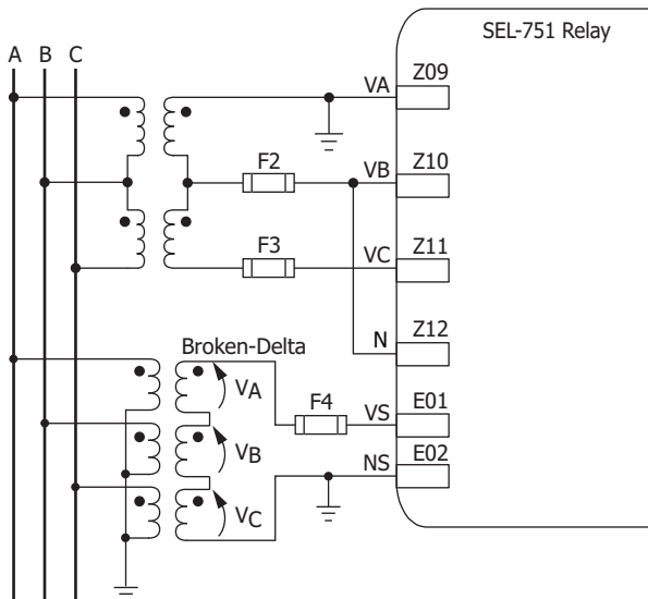
Figure 6 Broken-Delta Connections
