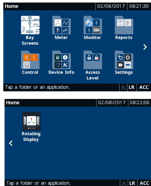
Figure 18 Home (Default FPHOME Screen)
