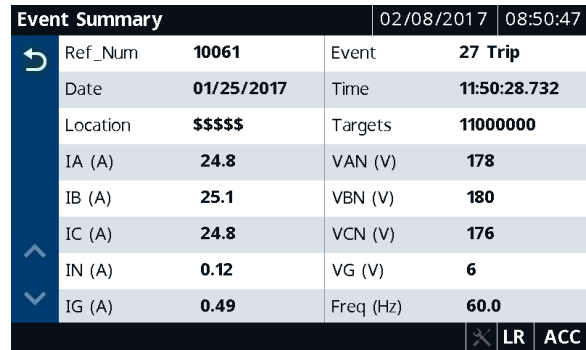
Figure 22 Event Summary
