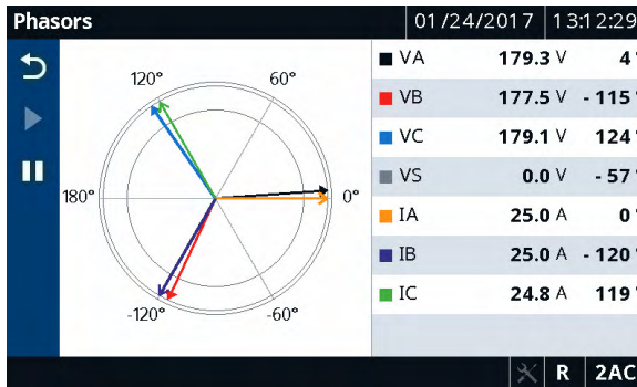
Figure 20 Meter Phasors
