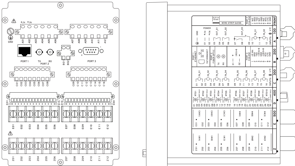
Figure 38 SEL-787-4X With Single Copper Ethernet, 8 DI, and RTD Option
