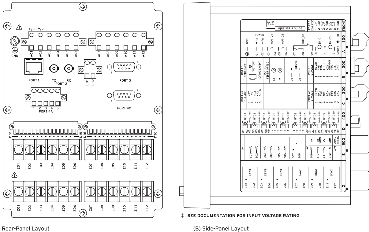
Figure 45 SEL-787-2E With Single Ethernet, EIA-232/EIA-485 Communications, and RTD Option
