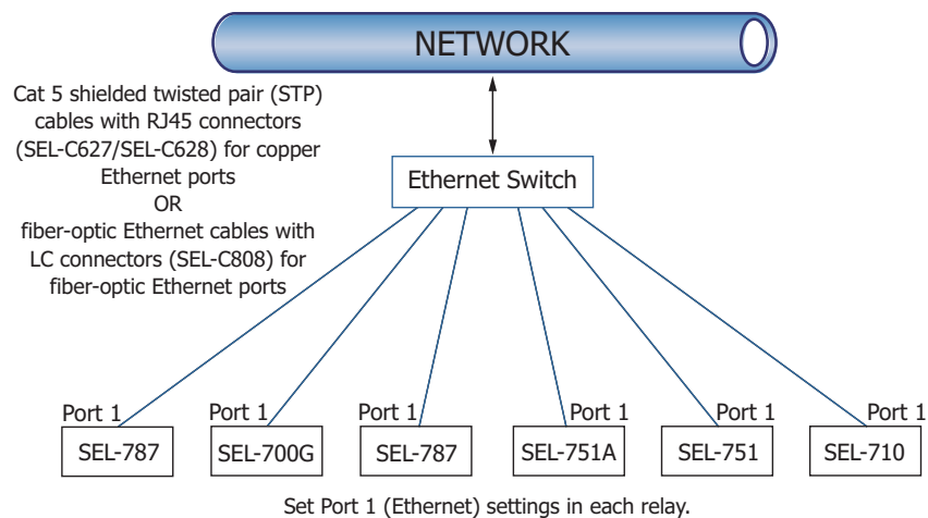
Figure 31 Simple Ethernet Network Configuration
