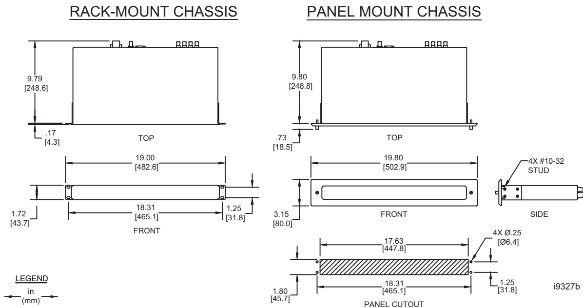
Figure 8 Dimensions for Rack- and Panel-Mount Models
