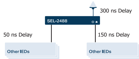
Figure 4 SEL-2488 Cable Delay Compensation
