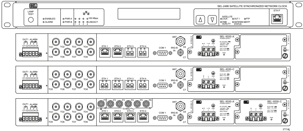
Figure 7 SEL-2488 Front and Rear Panels
