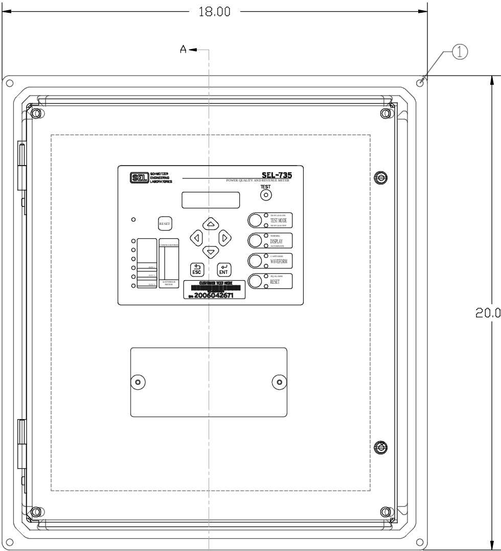
FRONT VIEW (FIBERGLASS ENC)
