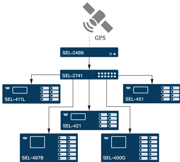
Figure 28 Example PTP Network
