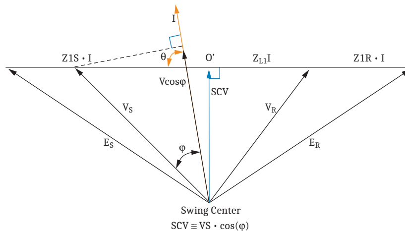
Figure 11 Applying V_S to Approximate the Swing Center Voltage Provides an Accurate Local Quantity to Detect Power Swings
