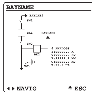
Figure 21 Ring Bus With Ground Switch
