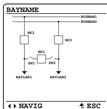
Figure 20 Breaker-and-a-Half
