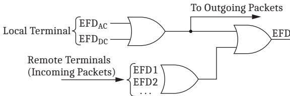
Figure 5 Combined External Fault Detector
