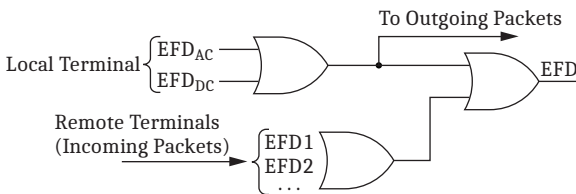
Figure 5 Combined External Fault Detector
