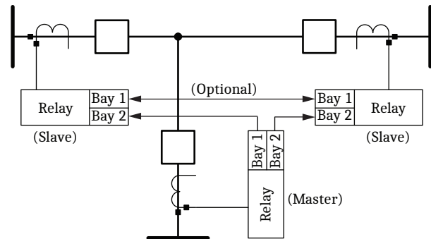
Figure 14 Three-Terminal 3SM Configuration With All Relays as Masters
