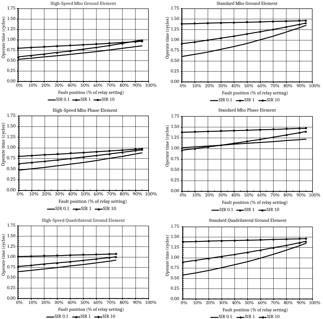
Figure 9 Distance Zone 1 Median Operating Time for Varying Fault Locations and Different SIRs
