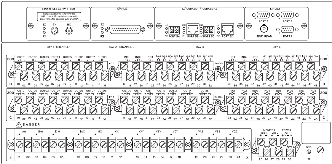
Figure 35 5U Rear Panel, Terminal Block, Two (INTD and INT7) I/O Board Option
