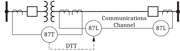
Figure 16 Preferred Application for Lines With Transformer
