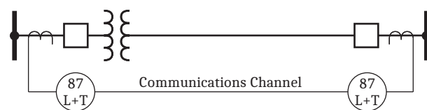
Figure 17 In-Line Transformer With Combined Line and Transformer Current Differential
