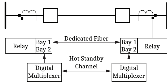
Figure 13 Two-Terminal Application With Hot Standby Channel
