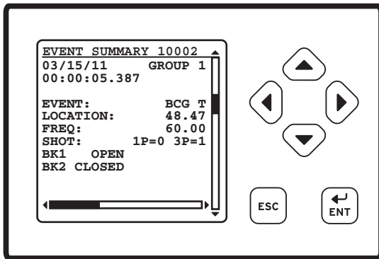
Figure 19 Factory-Default Front-Panel Display and Pushbuttons
