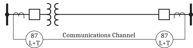
Figure 17 In-Line Transformer With Combined Line and Transformer Current Differential
