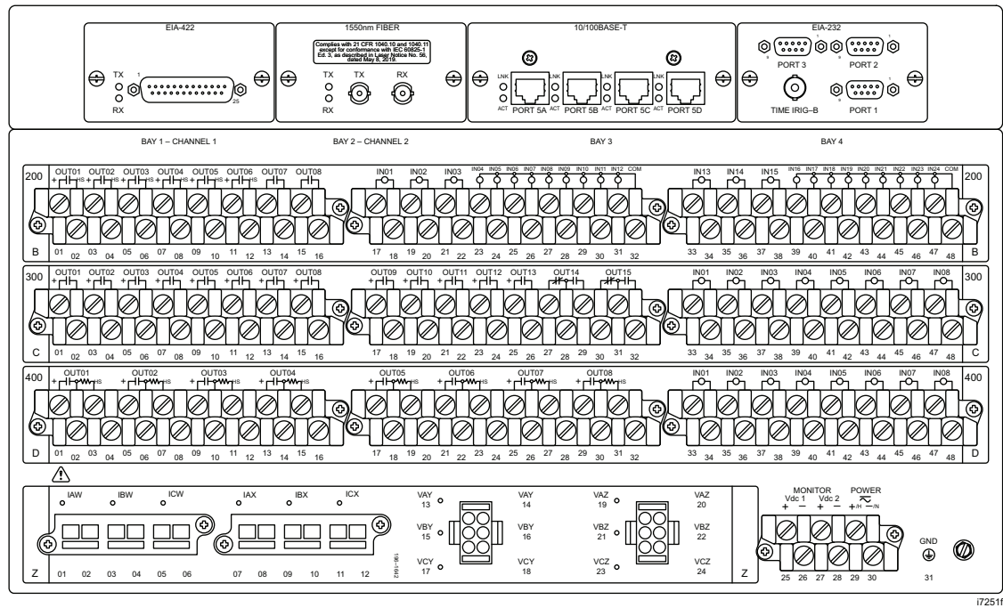
Figure 36 6U Rear Panel, Connectorized Terminal Block, Three (INTC, INT7, and INTE) I/O Board Option
