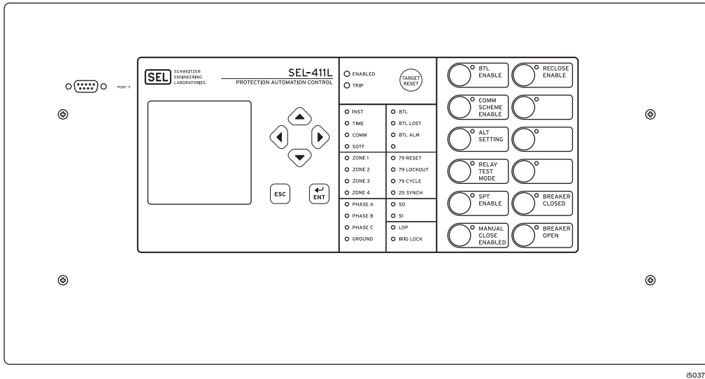
Figure 33 5U Front Panel, Panel-Mount Option
