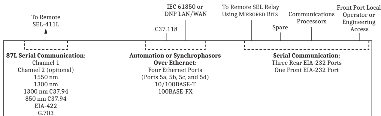
Figure 27 System Functional Overview
