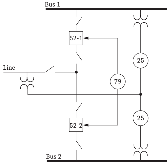
Figure 12 Two-Breaker Reclosing With Synchronism Check
