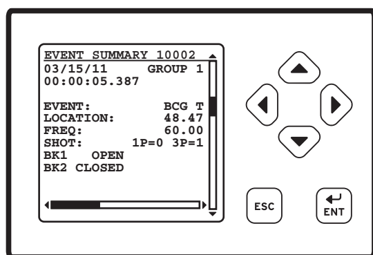
Figure 19 Factory-Default Front-Panel Display and Pushbuttons
