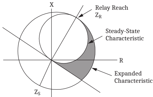
Figure 10 Mho Characteristic
