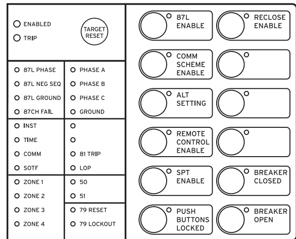
Figure 18 Factory Default Status and Trip Target LEDs (12 Pushbutton, 24 Target LED Option)
