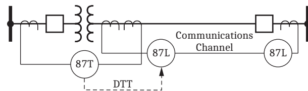
Figure 16 Preferred Application for Lines With Transformer
