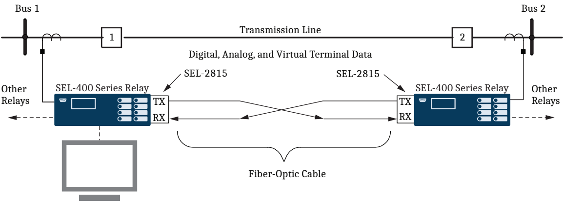
Figure 29 Integral Communication Provides Secure Protection, Monitoring, and Control as Well as Terminal Access to Both Relays Through One Connection
