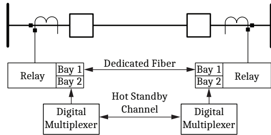
Figure 13 Two-Terminal Application With Hot Standby Channel
