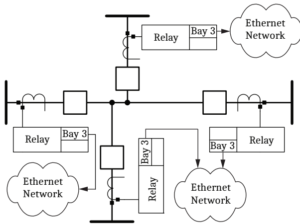
Figure 15 Four-Terminal Ethernet Application
