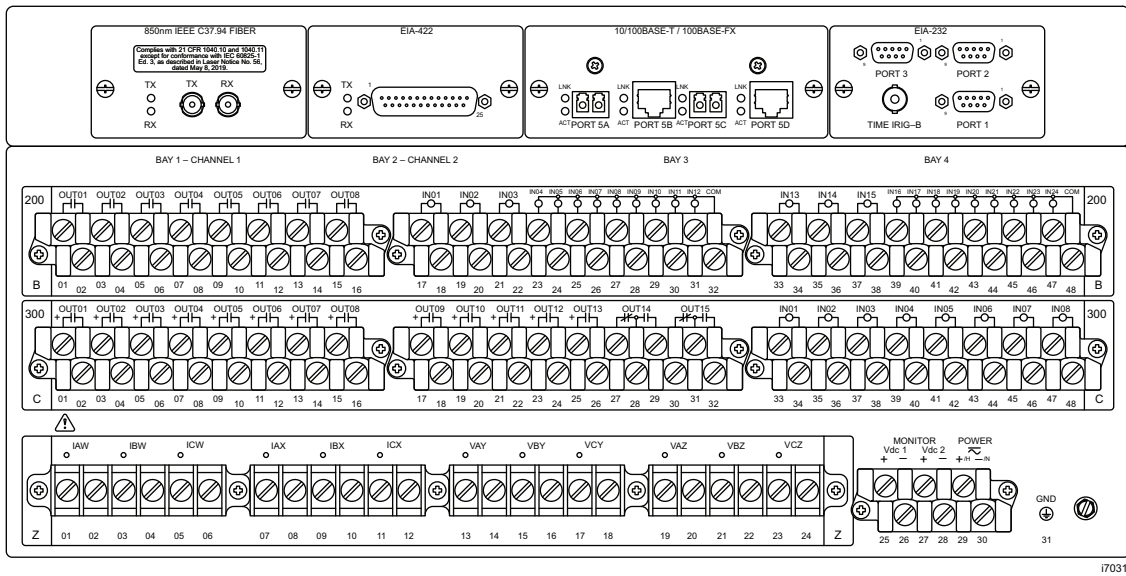
Figure 35 5U Rear Panel, Terminal Block, Two (INTD and INT7) I/O Board Option
