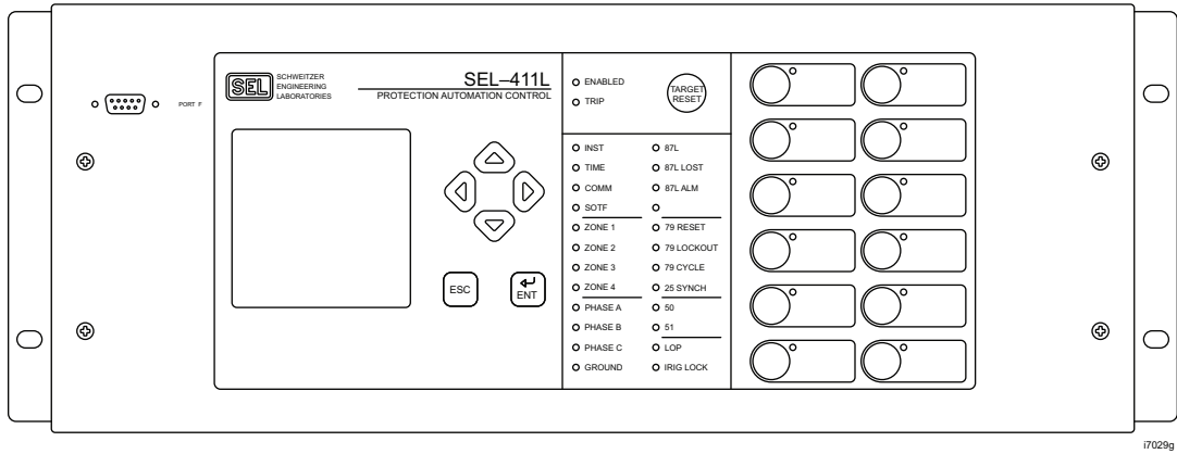
Figure 32 4U Front Panel, Rack-Mount Option
