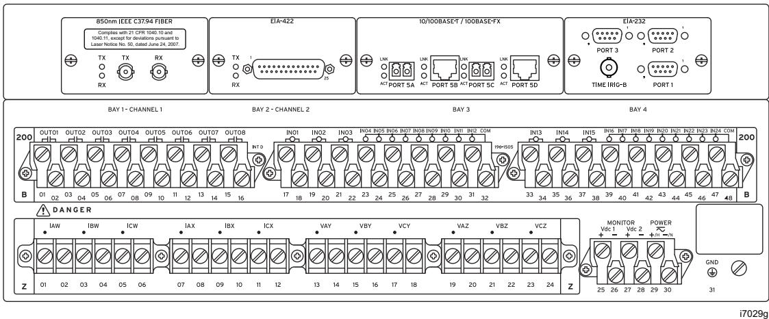
Figure 34 4U Rear Panel, Terminal Block, One (INTD) I/O Board Option
