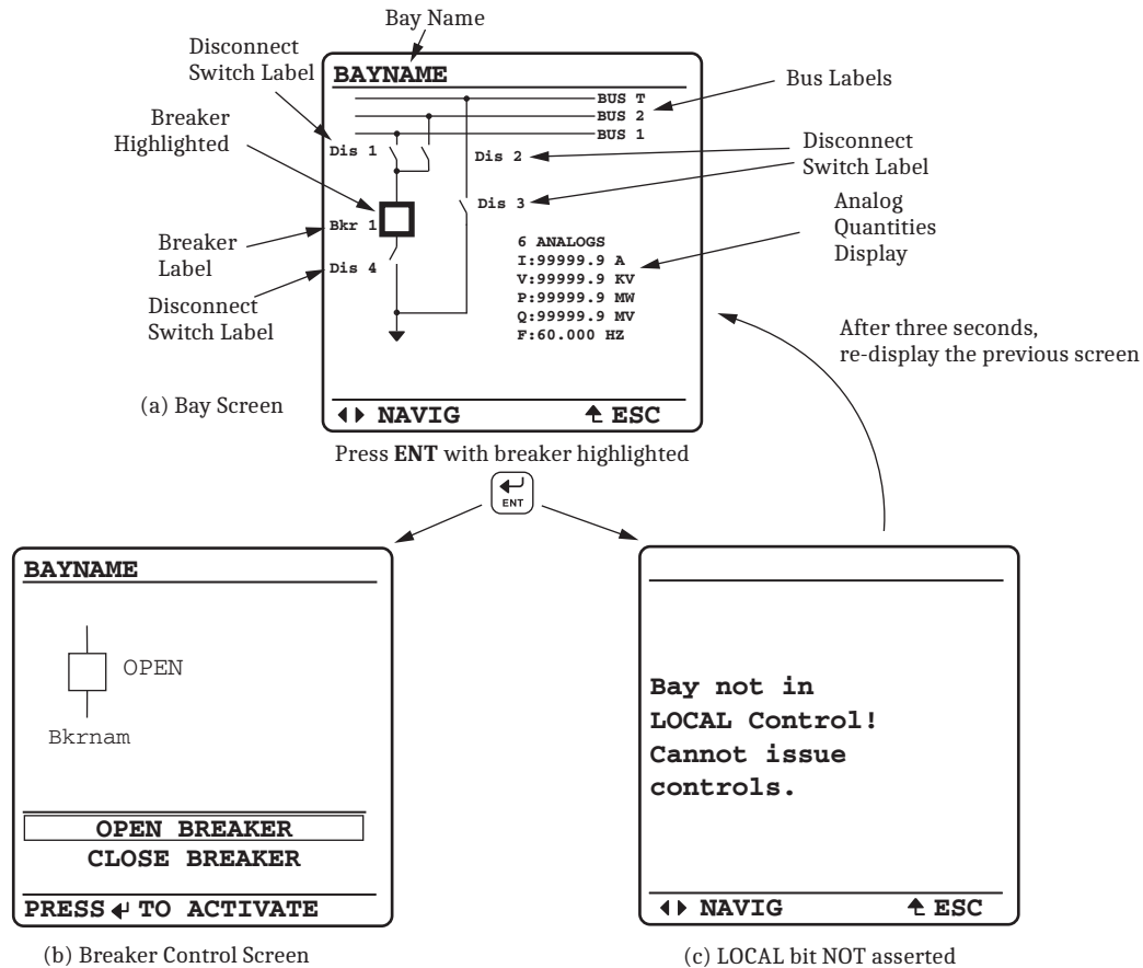
Figure 24 Screens for Circuit Breaker Selection
