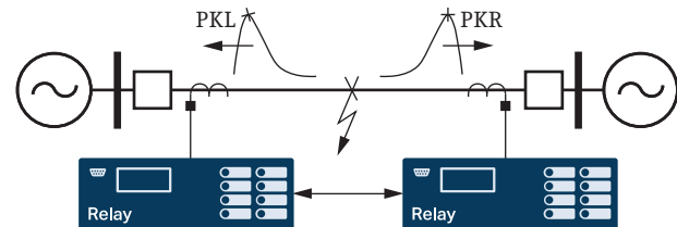
Figure 31 Relays Exchanging Peak Information Via 87L Communications Channel
