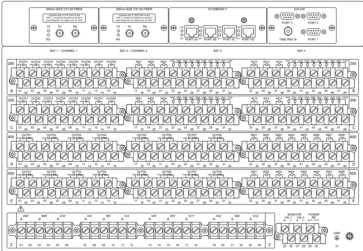
Figure 37 7U Rear Panel, Terminal Block, Four (Two INT4 and Two INT8) I/O Board Option
