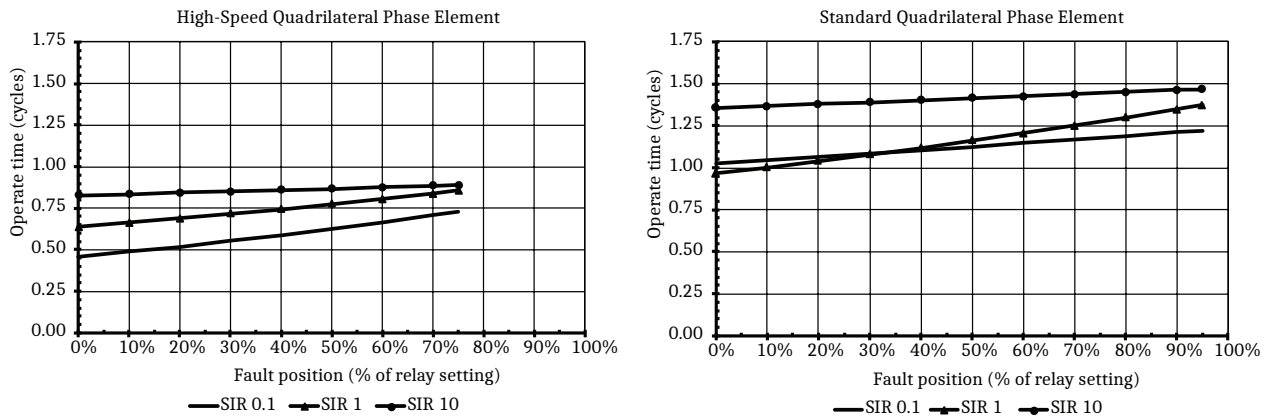
Figure 9 Distance Zone 1 Median Operating Time for Varying Fault Locations and Different SIRs (Continued)
