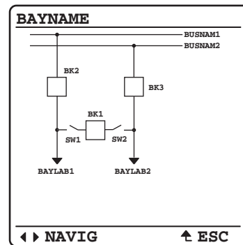
Figure 20 Breaker-and-a-Half
