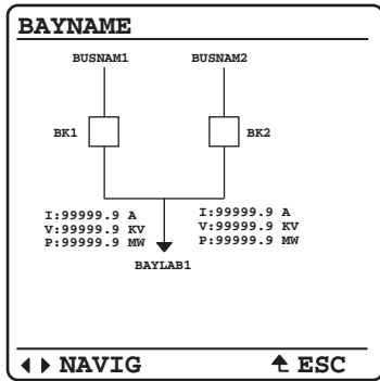
Figure 23 Source Transfer Bus
