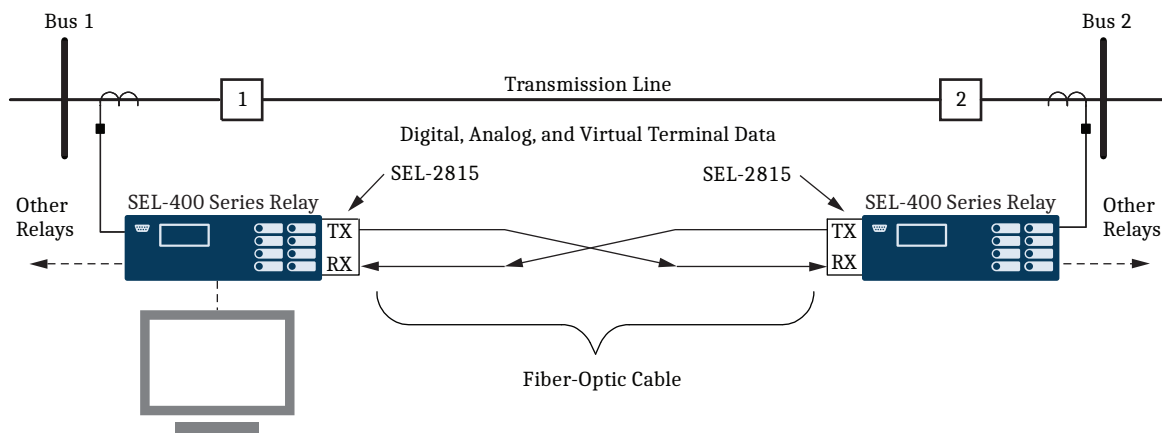
Figure 29 Integral Communication Provides Secure Protection, Monitoring, and Control as Well as Terminal Access to Both Relays Through One Connection
