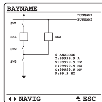
Figure 22 Double Bus/Double Breaker
