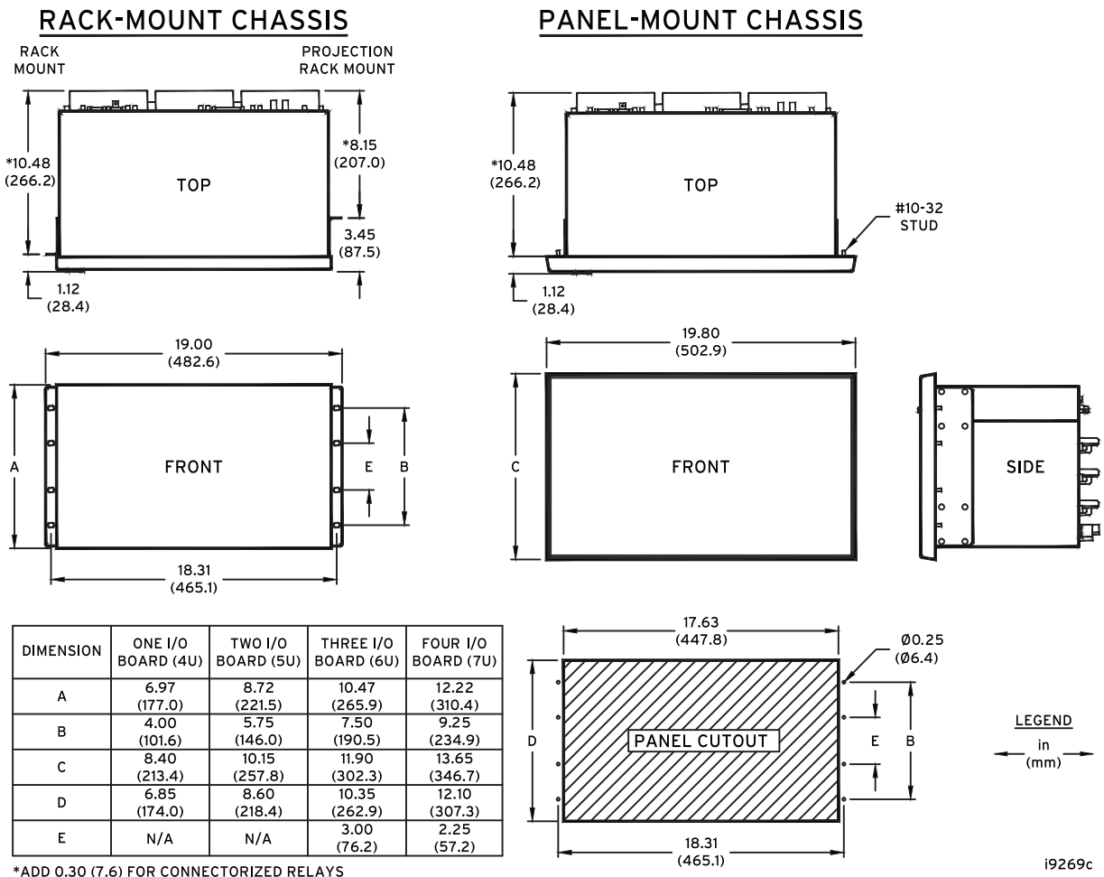
Figure 38 4U, 5U, 6U, and 7U Chassis Dimensions
