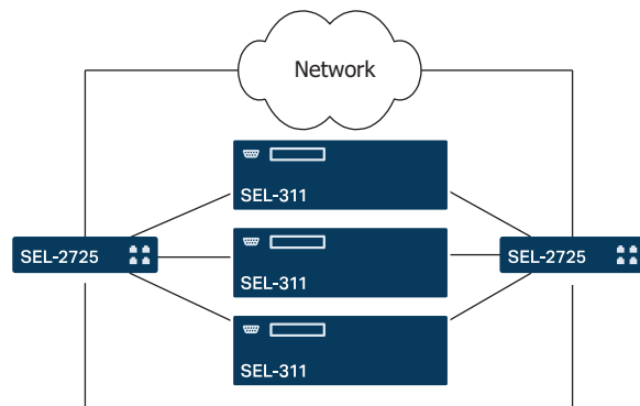
Figure 19 Failover Network Topology
