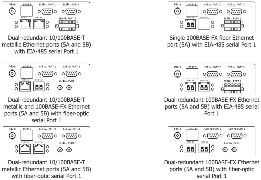
Figure 28 SEL-311C Rear-Panel Communications Port Configurations
