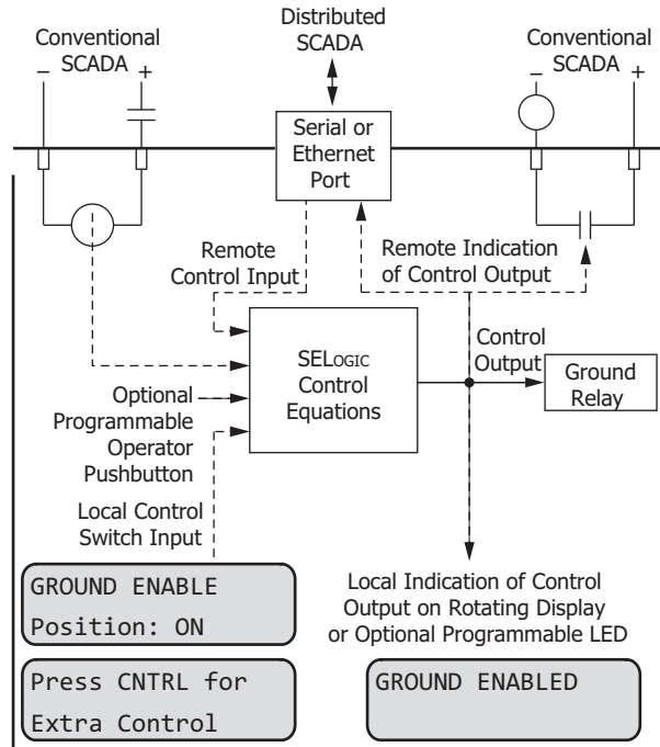
Figure 13 Local and Remote Control Using SELogic Control Equations (Ground Relay Example)
