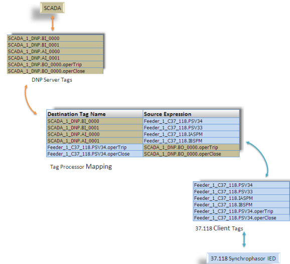
Figure 2 Map Synchronphasor Data Seamlessly Into SCADA Connections
