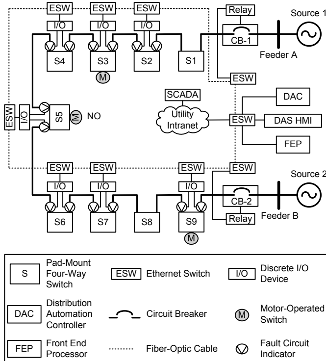
Fig. 1. Typical Automated Dual Distribution Feeder-Looped Circuit
