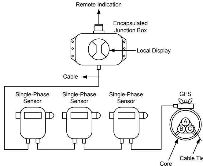
Fig. 2. Four-Sensor FCI
